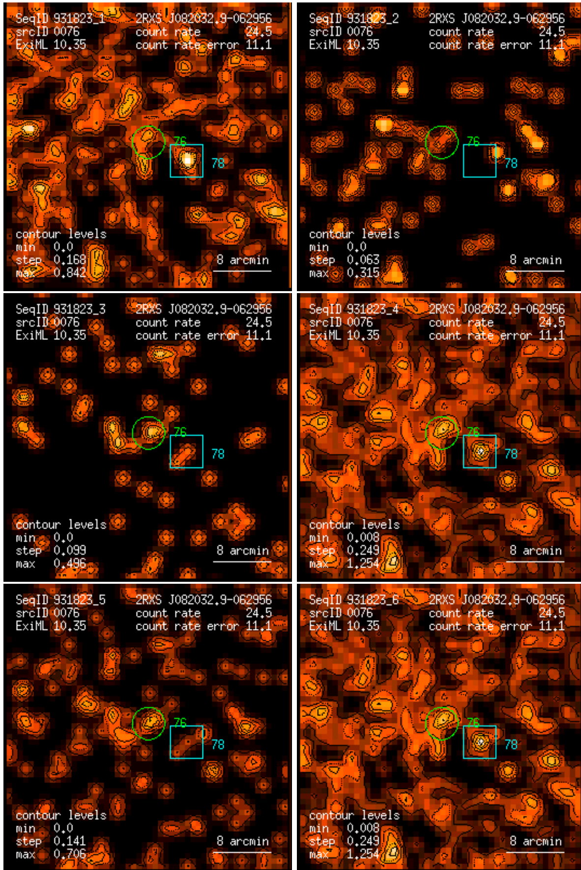
Figure 76: RASS 931823: detection 0076: band rate images, Gaussian filter: (1) PSPC channels 11 – 41, (2) 52 – 90, (3) 91 – 201, (4) 11 – 235, (5) 52 – 201, (6) 11 – 201. Broad band rates in counts/ks. Band rate contour levels in counts/ks/arcmin 2 .
