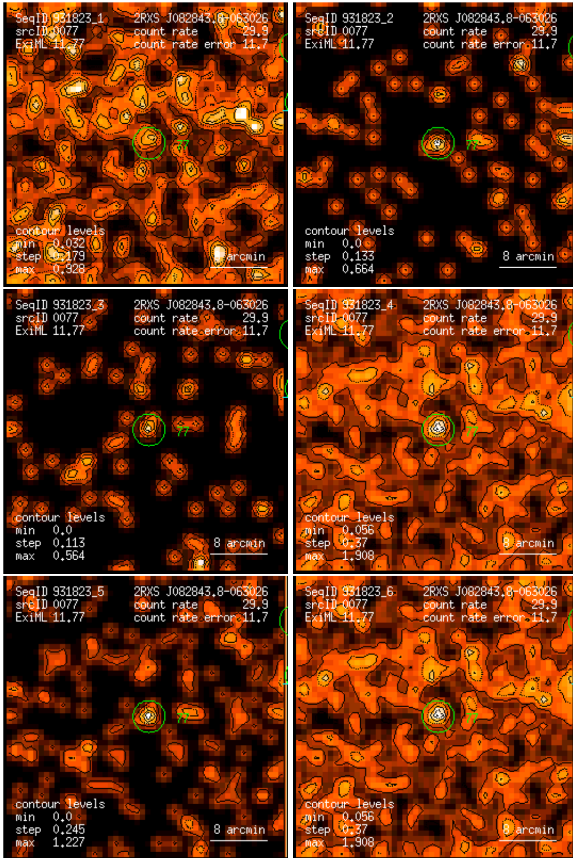
Figure 77: RASS 931823: detection 0077: band rate images, Gaussian filter: (1) PSPC channels 11 – 41, (2) 52 – 90, (3) 91 – 201, (4) 11 – 235, (5) 52 – 201, (6) 11 – 201. Broad band rates in counts/ks. Band rate contour levels in counts/ks/arcmin 2 .
