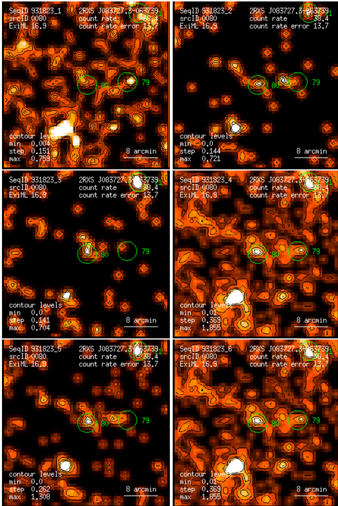
Figure 80: RASS 931823: detection 0080: band rate images, Gaussian filter: (1) PSPC channels 11 – 41, (2) 52 – 90, (3) 91 – 201, (4) 11 – 235, (5) 52 – 201, (6) 11 – 201. Broad band rates in counts/ks. Band rate contour levels in counts/ks/arcmin 2 .
