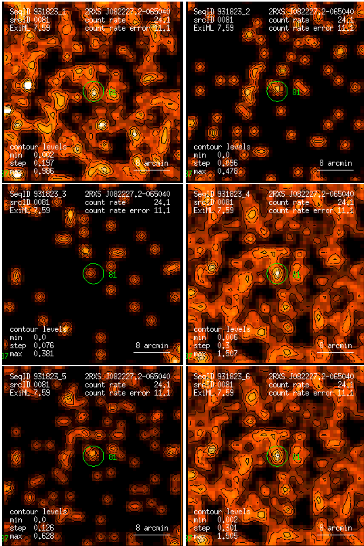
Figure 81: RASS 931823: detection 0081: band rate images, Gaussian filter: (1) PSPC channels 11 – 41, (2) 52 – 90, (3) 91 – 201, (4) 11 – 235, (5) 52 – 201, (6) 11 – 201. Broad band rates in counts/ks. Band rate contour levels in counts/ks/arcmin 2 .
