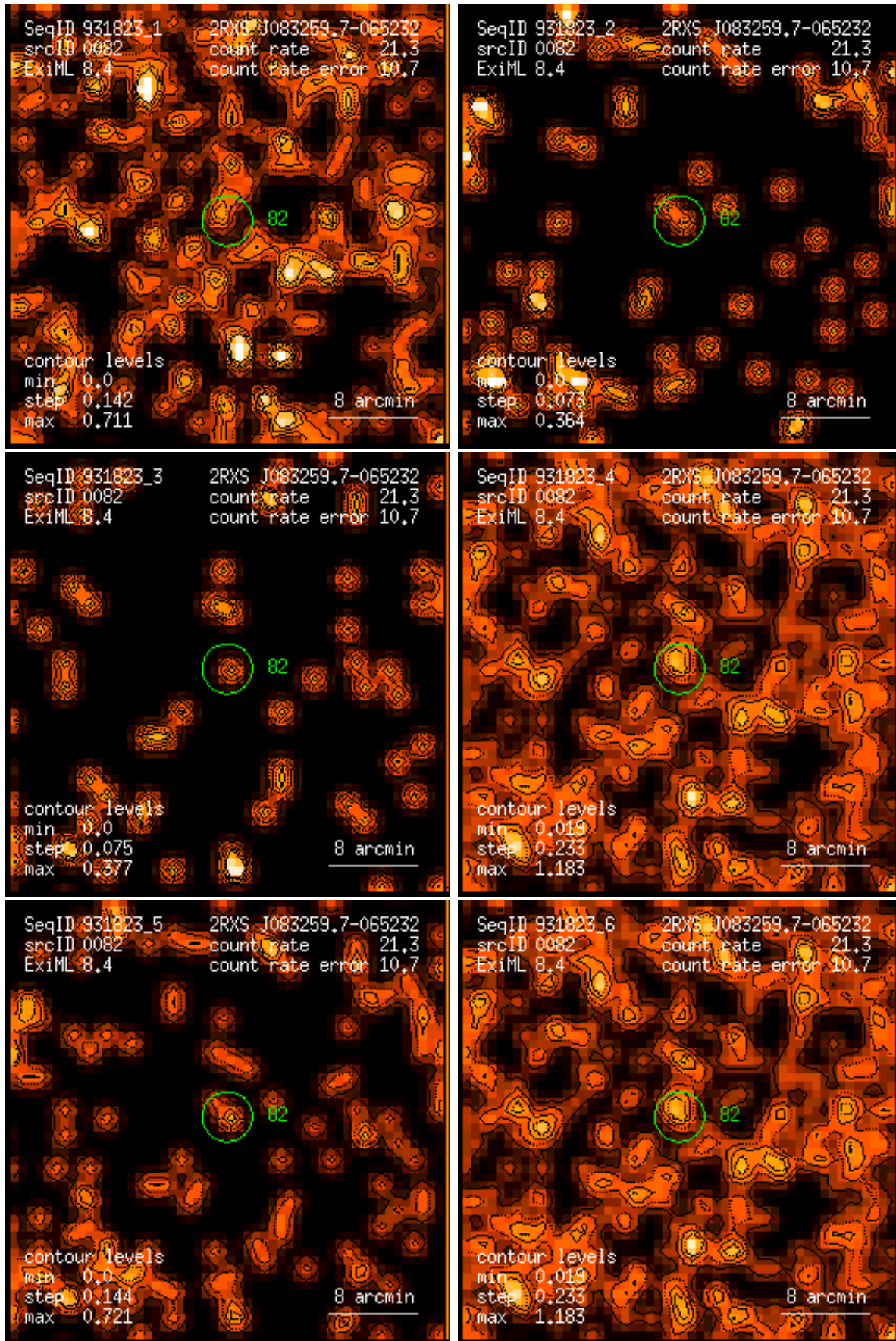
Figure 82: RASS 931823: detection 0082: band rate images, Gaussian filter: (1) PSPC channels 11 – 41, (2) 52 – 90, (3) 91 – 201, (4) 11 – 235, (5) 52 – 201, (6) 11 – 201. Broad band rates in counts/ks. Band rate contour levels in counts/ks/arcmin 2 .
