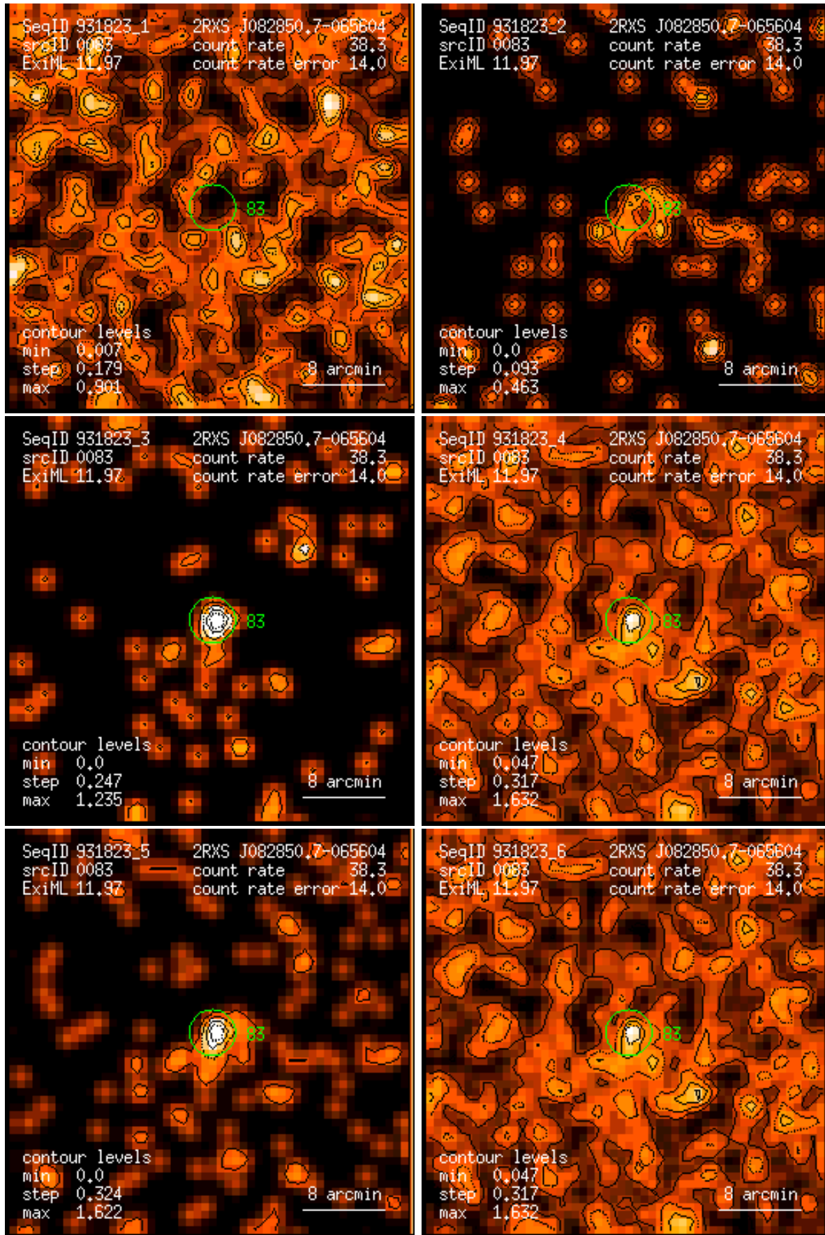
Figure 83: RASS 931823: detection 0083: band rate images, Gaussian filter: (1) PSPC channels 11 – 41, (2) 52 – 90, (3) 91 – 201, (4) 11 – 235, (5) 52 – 201, (6) 11 – 201. Broad band rates in counts/ks. Band rate contour levels in counts/ks/arcmin 2 .
