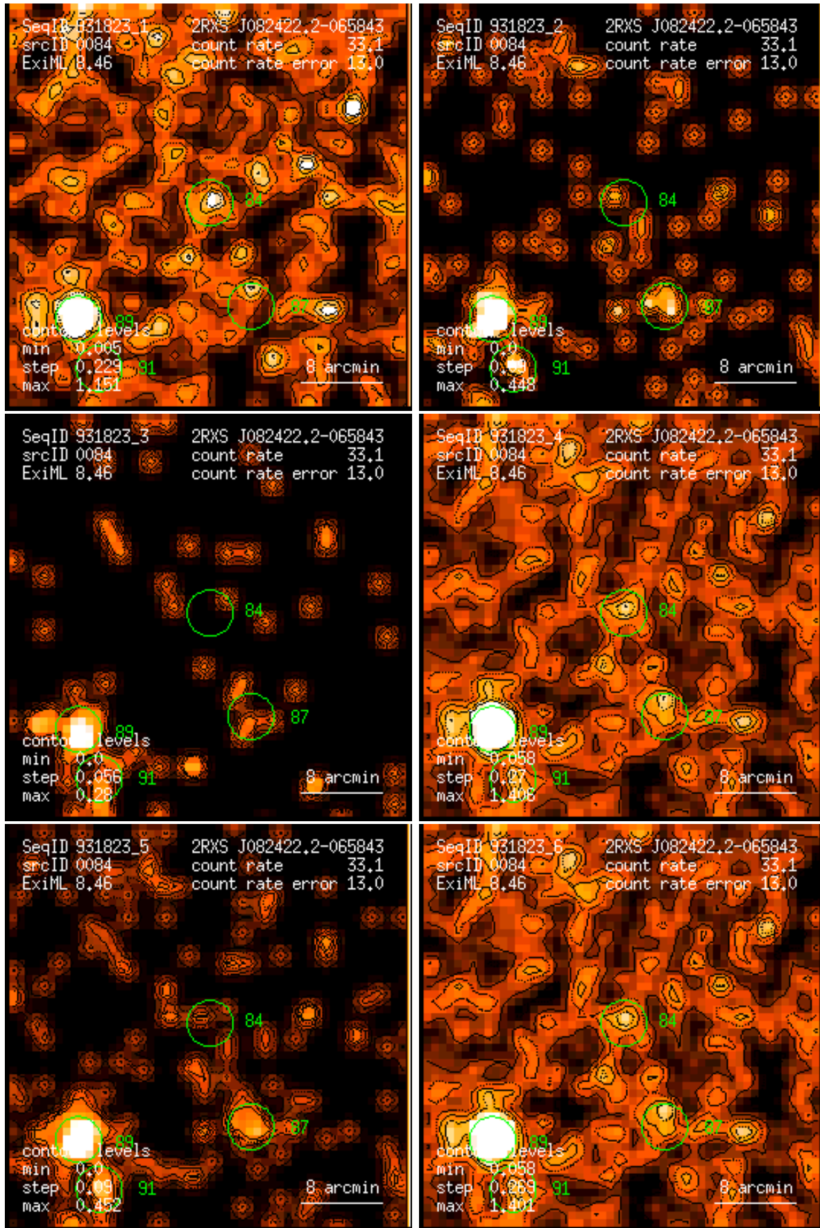
Figure 84: RASS 931823: detection 0084: band rate images, Gaussian filter: (1) PSPC channels 11 – 41, (2) 52 – 90, (3) 91 – 201, (4) 11 – 235, (5) 52 – 201, (6) 11 – 201. Broad band rates in counts/ks. Band rate contour levels in counts/ks/arcmin 2 .
