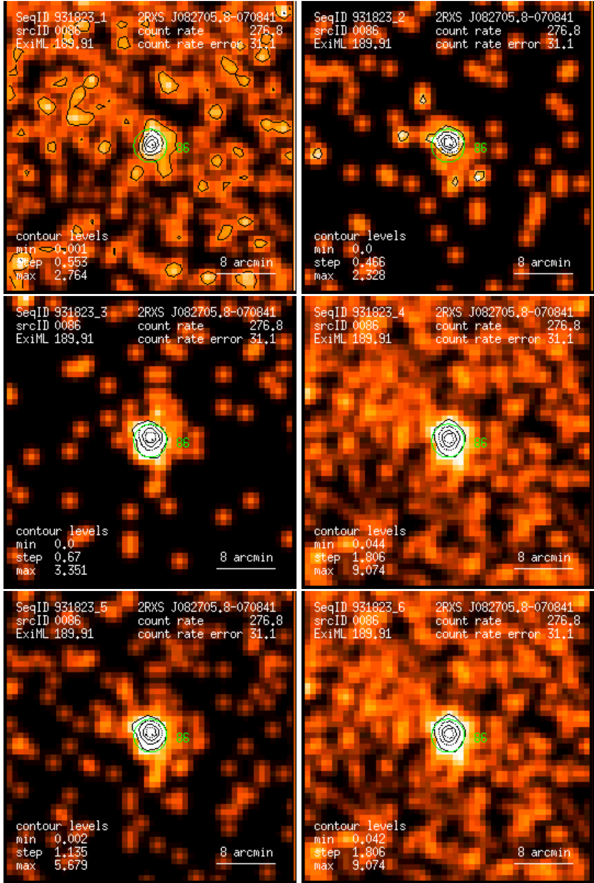
Figure 86: RASS 931823: detection 0086: band rate images, Gaussian filter: (1) PSPC channels 11 – 41, (2) 52 – 90, (3) 91 – 201, (4) 11 – 235, (5) 52 – 201, (6) 11 – 201. Broad band rates in counts/ks. Band rate contour levels in counts/ks/arcmin 2 .
