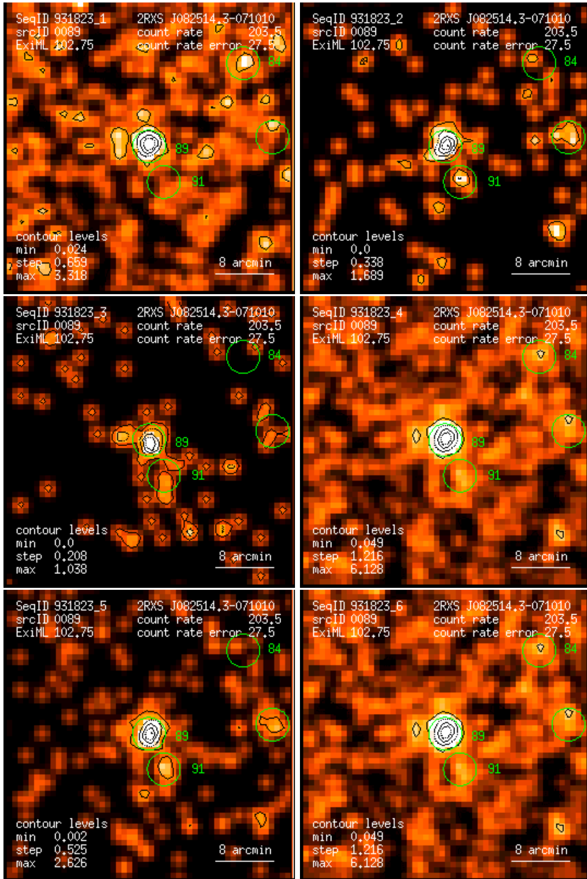
Figure 89: RASS 931823: detection 0089: band rate images, Gaussian filter: (1) PSPC channels 11 – 41, (2) 52 – 90, (3) 91 – 201, (4) 11 – 235, (5) 52 – 201, (6) 11 – 201. Broad band rates in counts/ks. Band rate contour levels in counts/ks/arcmin 2 .
