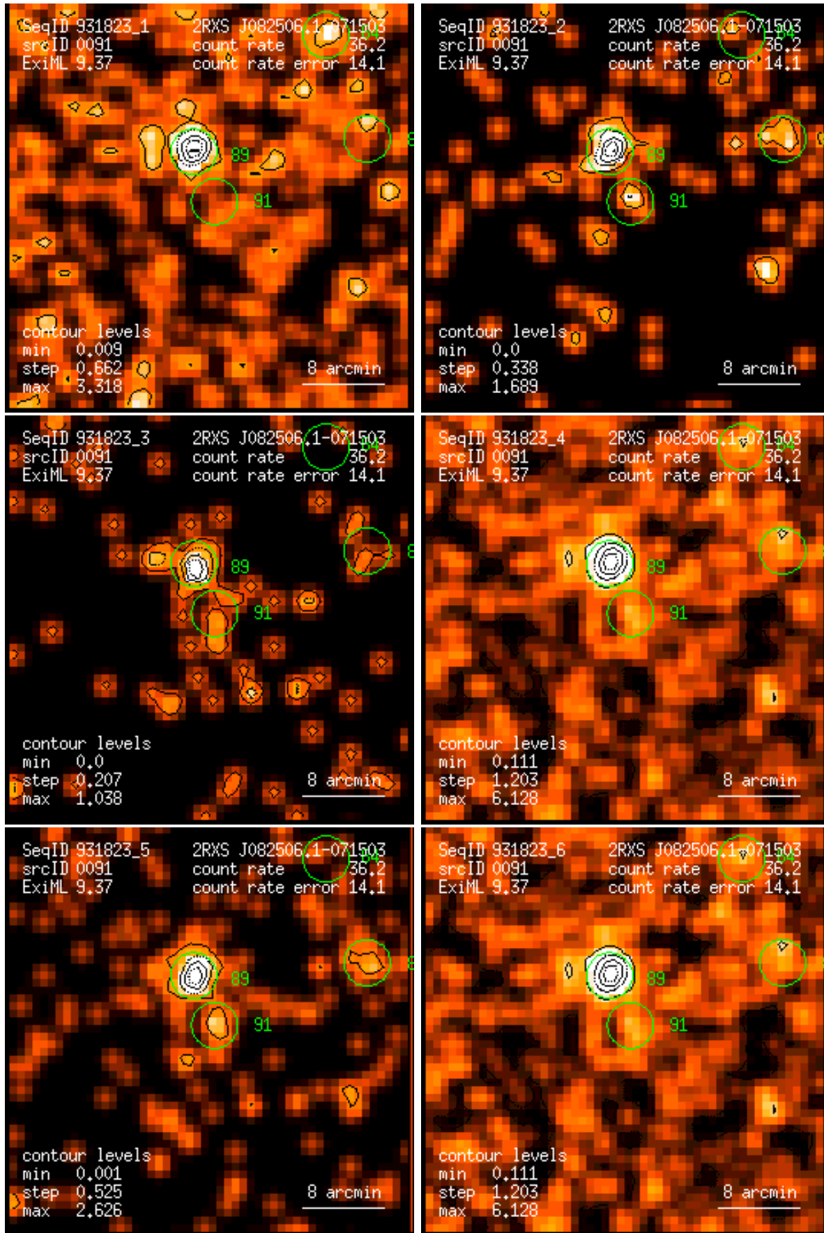
Figure 91: RASS 931823: detection 0091: band rate images, Gaussian filter: (1) PSPP channels 11 – 41, (2) 52 – 90, (3) 91 – 201, (4) 11 – 235, (5) 52 – 201, (6) 11 – 201. Broad band rates in counts/ks. Band rate contour levels in counts/ks/arcmin 2 .
