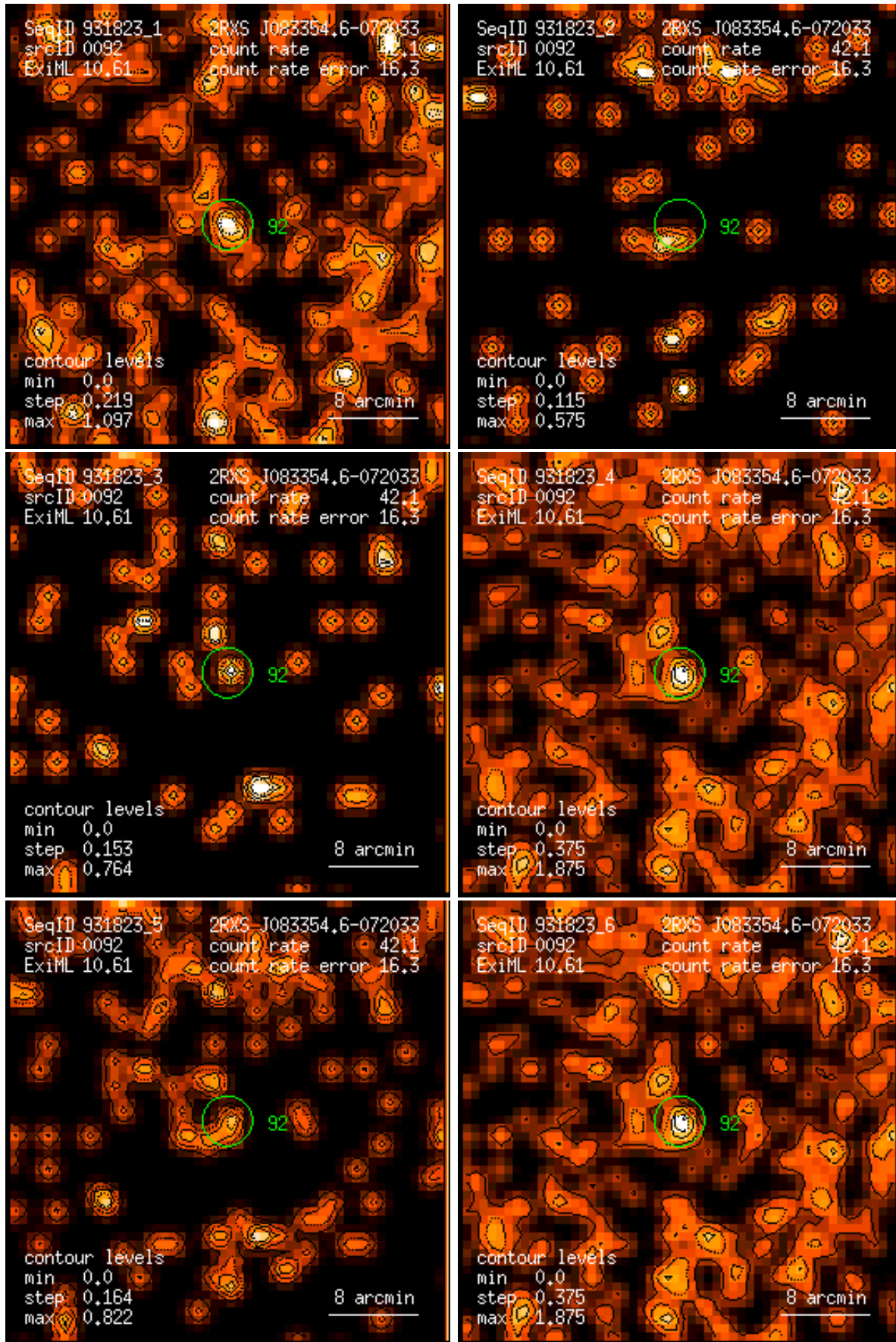
Figure 92: RASS 931823: detection 0092: band rate images, Gaussian filter: (1) PSPC channels 11 – 41, (2) 52 – 90, (3) 91 – 201, (4) 11 – 235, (5) 52 – 201, (6) 11 – 201. Broad band rates in counts/ks. Band rate contour levels in counts/ks/arcmin 2 .
