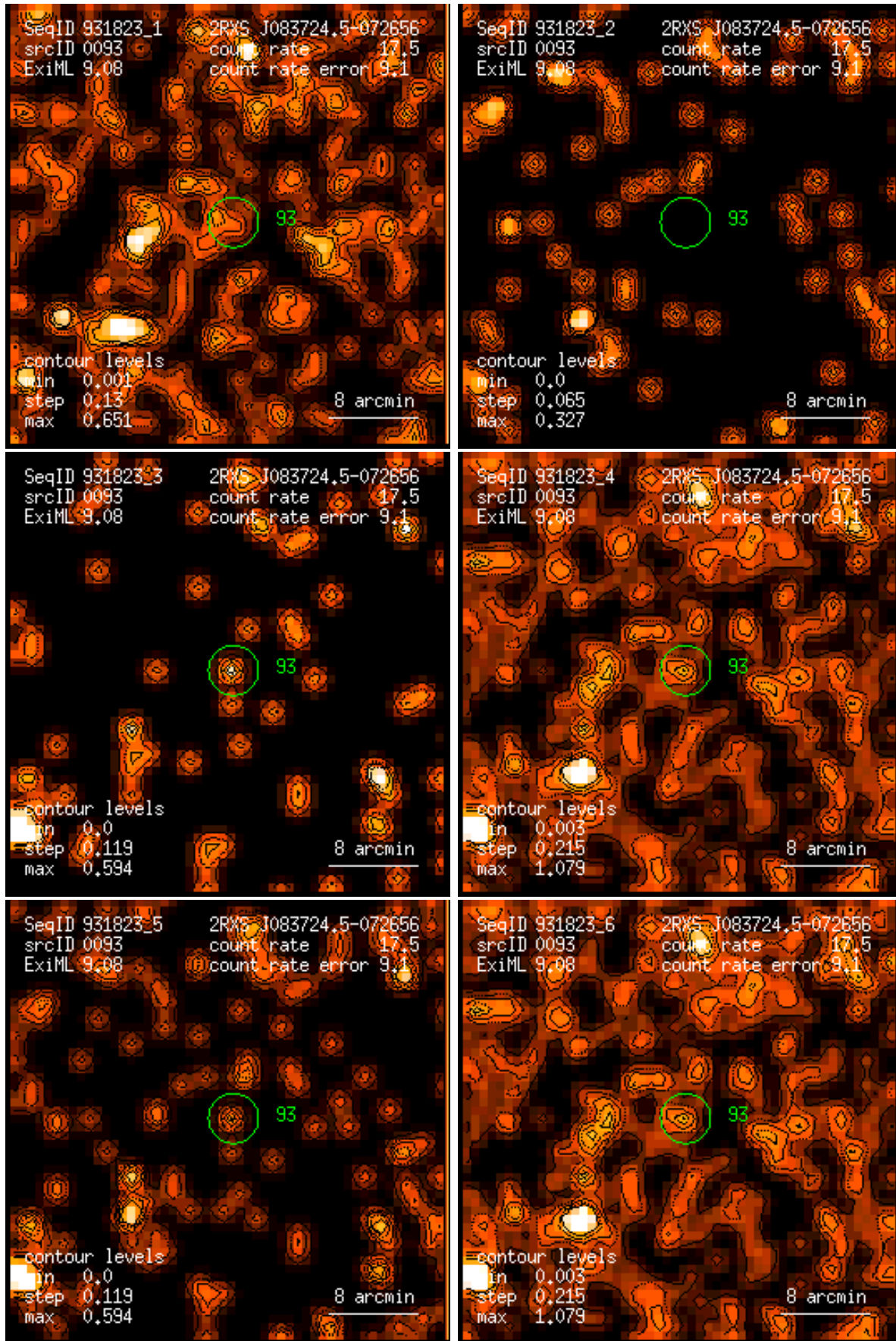
Figure 93: RASS 931823: detection 0093: band rate images, Gaussian filter: (1) PSPC channels 11 – 41, (2) 52 – 90, (3) 91 – 201, (4) 11 – 235, (5) 52 – 201, (6) 11 – 201. Broad band rates in counts/ks. Band rate contour levels in counts/ks/arcmin 2 .
