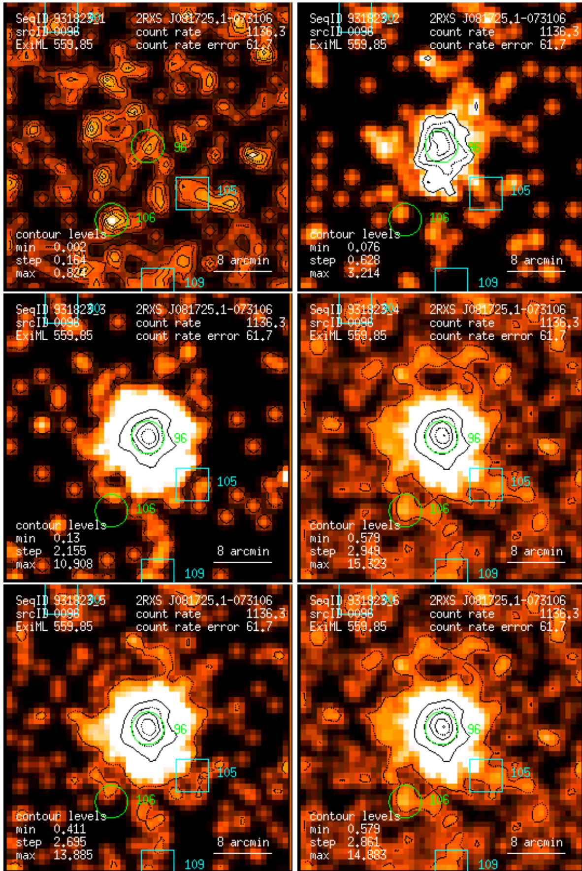
Figure 96: RASS 931823: detection 0096: band rate images, Gaussian filter: (1) PSPC channels 11 – 41, (2) 52 – 90, (3) 91 – 201, (4) 11 – 235, (5) 52 – 201, (6) 11 – 201. Broad band rates in counts/ks. Band rate contour levels in counts/ks/arcmin 2 .
