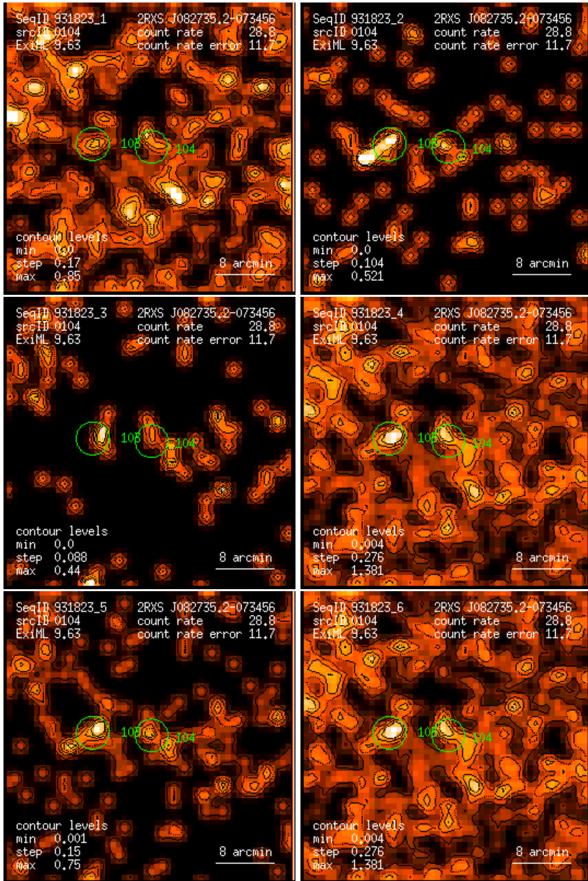
Figure 104: RASS 931823: detection 0104: band rate images, Gaussian filter: (1) PSPC channels 11 – 41, (2) 52 – 90, (3) 91 – 201, (4) 11 – 235, (5) 52 – 201, (6) 11 – 201. Broad band rates in counts/ks. Band rate contour levels in counts/ks/arcmin 2 .
