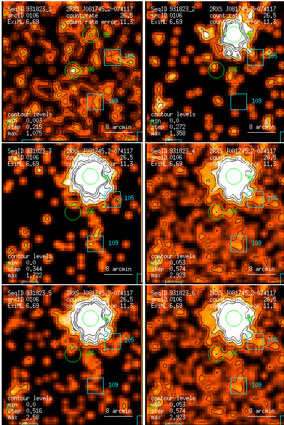
Figure 106: RASS 931823: detection 0106: band rate images, Gaussian filter: (1) PSPC channels 11 – 41, (2) 52 – 90, (3) 91 – 201, (4) 11 – 235, (5) 52 – 201, (6) 11 – 201. Broad band rates in counts/ks. Band rate contour levels in counts/ks/arcmin 2 .
