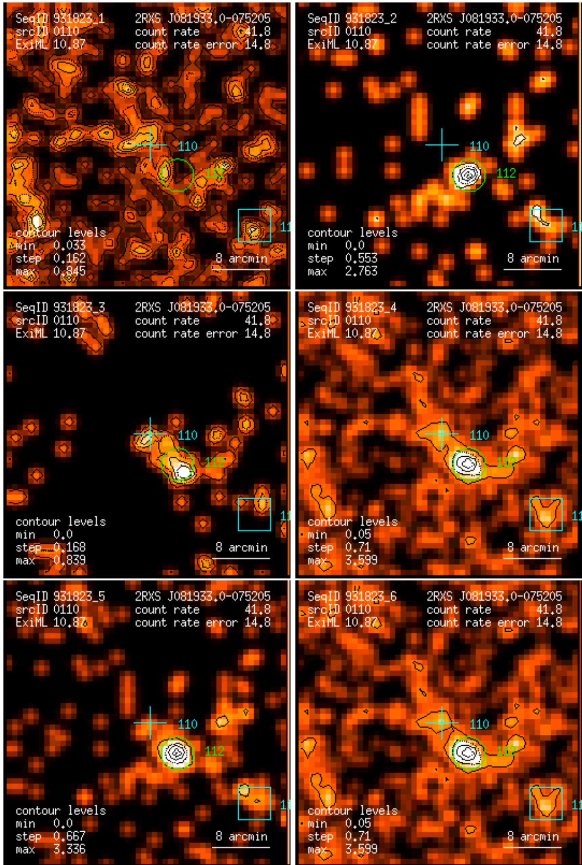
Figure 110: RASS 931823: detection 0110: band rate images, Gaussian filter: (1) PSPC channels 11 – 41, (2) 52 – 90, (3) 91 – 201, (4) 11 – 235, (5) 52 – 201, (6) 11 – 201. Broad band rates in counts/ks. Band rate contour levels in counts/ks/arcmin 2 .
