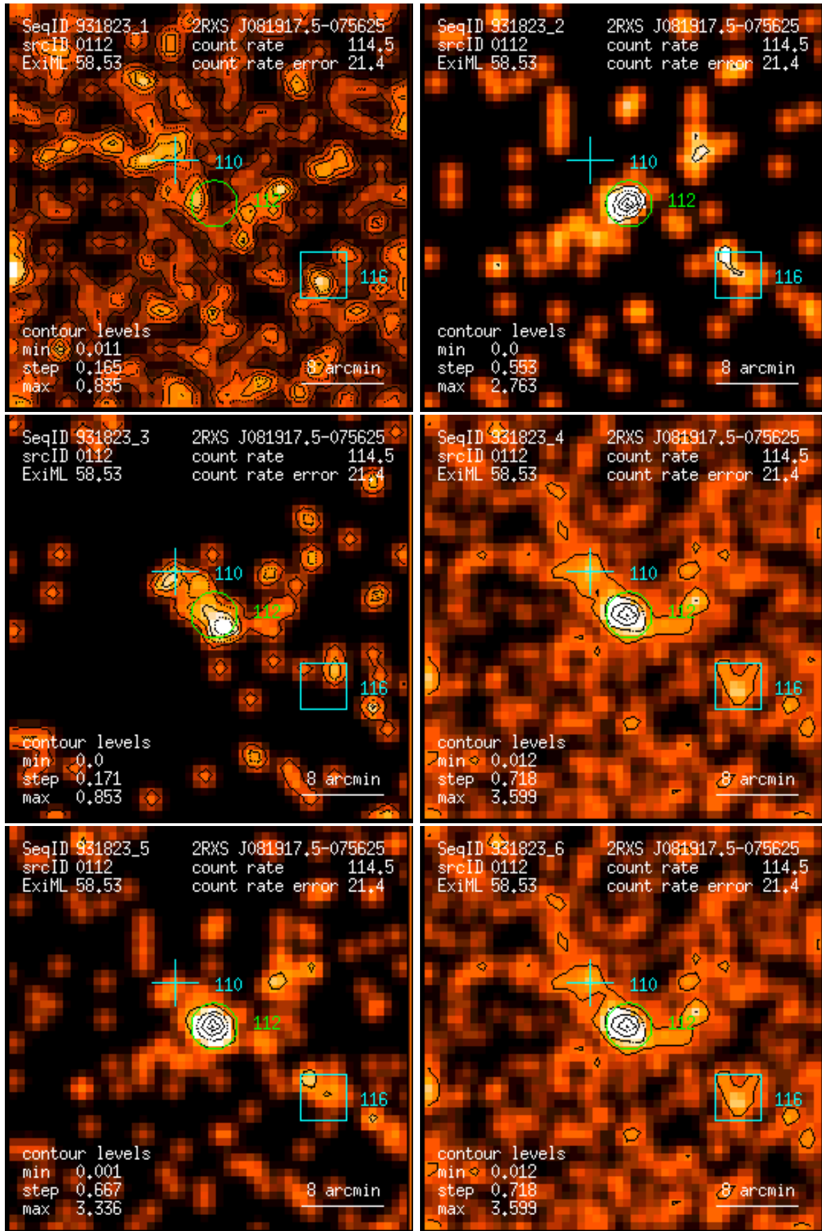
Figure 112: RASS 931823: detection 0112: band rate images, Gaussian filter: (1) PSPC channels 11 – 41, (2) 52 – 90, (3) 91 – 201, (4) 11 – 235, (5) 52 – 201, (6) 11 – 201. Broad band rates in counts/ks. Band rate contour levels in counts/ks/arcmin 2 .
