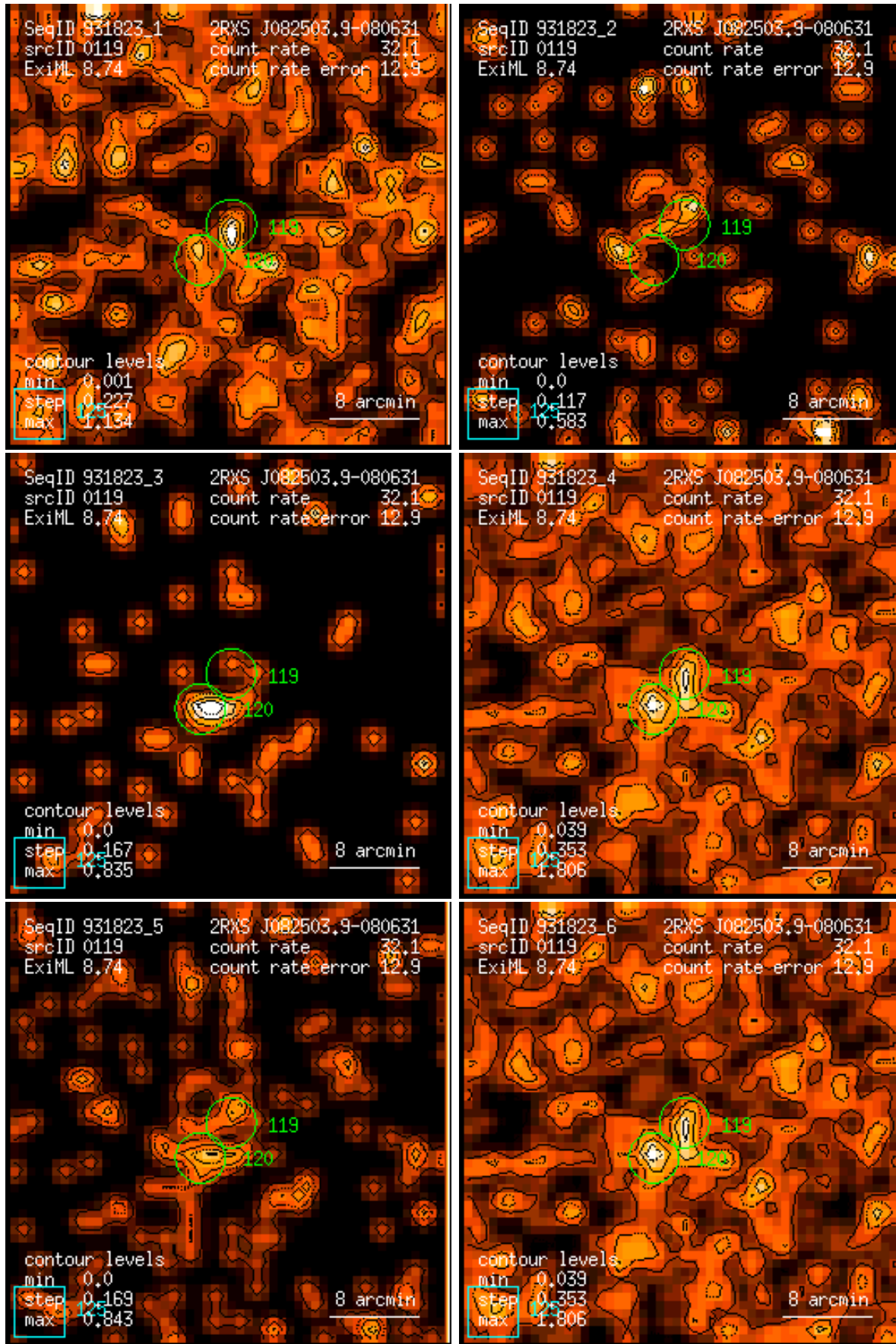
Figure 119: RASS 931823: detection 0119: band rate images, Gaussian filter: (1) PSPC channels 11 – 41, (2) 52 – 90, (3) 91 – 201, (4) 11 – 235, (5) 52 – 201, (6) 11 – 201. Broad band rates in counts/ks. Band rate contour levels in counts/ks/arcmin 2 .
