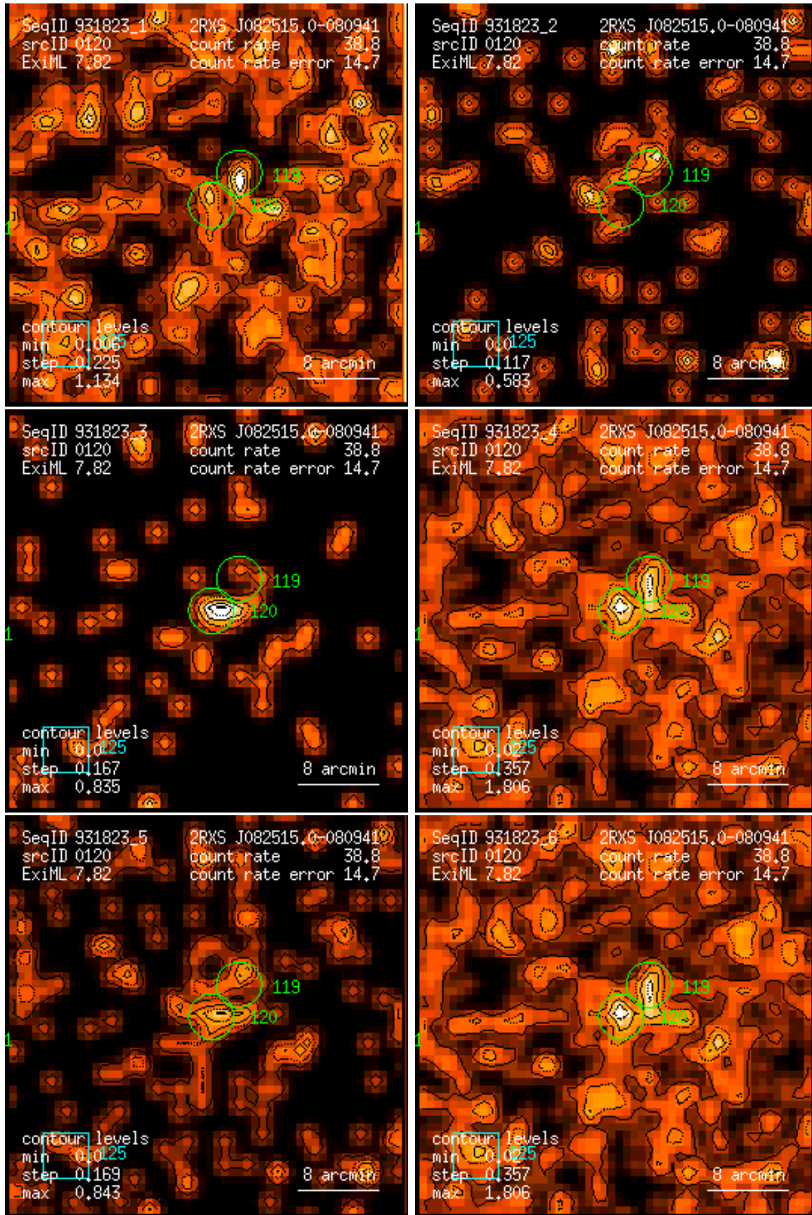
Figure 120: RASS 931823: detection 0120: band rate images, Gaussian filter: (1) PSPC channels 11 – 41, (2) 52 – 90, (3) 91 – 201, (4) 11 – 235, (5) 52 – 201, (6) 11 – 201. Broad band rates in counts/ks. Band rate contour levels in counts/ks/arcmin 2 .
