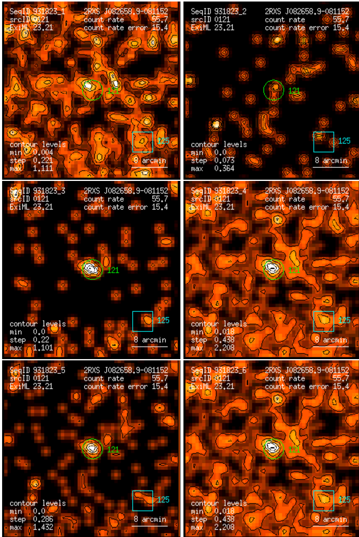
Figure 121: RASS 931823: detection 0121: band rate images, Gaussian filter: (1) PSPC channels 11 – 41, (2) 52 – 90, (3) 91 – 201, (4) 11 – 235, (5) 52 – 201, (6) 11 – 201. Broad band rates in counts/ks. Band rate contour levels in counts/ks/arcmin 2 .
