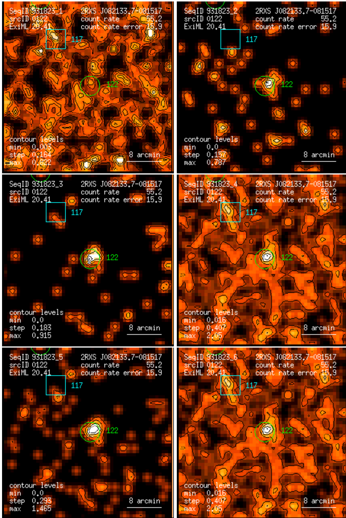
Figure 122: RASS 931823: detection 0122: band rate images, Gaussian filter: (1) PSPC channels 11 – 41, (2) 52 – 90, (3) 91 – 201, (4) 11 – 235, (5) 52 – 201, (6) 11 – 201. Broad band rates in counts/ks. Band rate contour levels in counts/ks/arcmin 2 .
