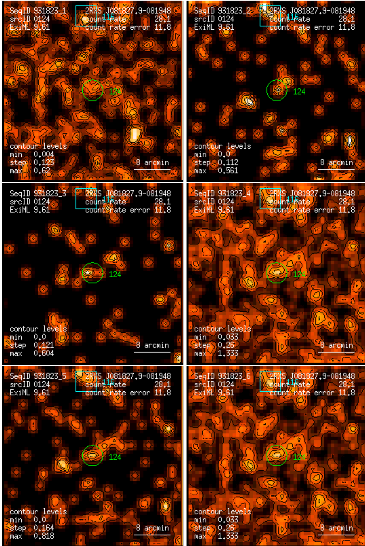
Figure 124: RASS 931823: detection 0124: band rate images, Gaussian filter: (1) PSPC channels 11 – 41, (2) 52 – 90, (3) 91 – 201, (4) 11 – 235, (5) 52 – 201, (6) 11 – 201. Broad band rates in counts/ks. Band rate contour levels in counts/ks/arcmin 2 .
