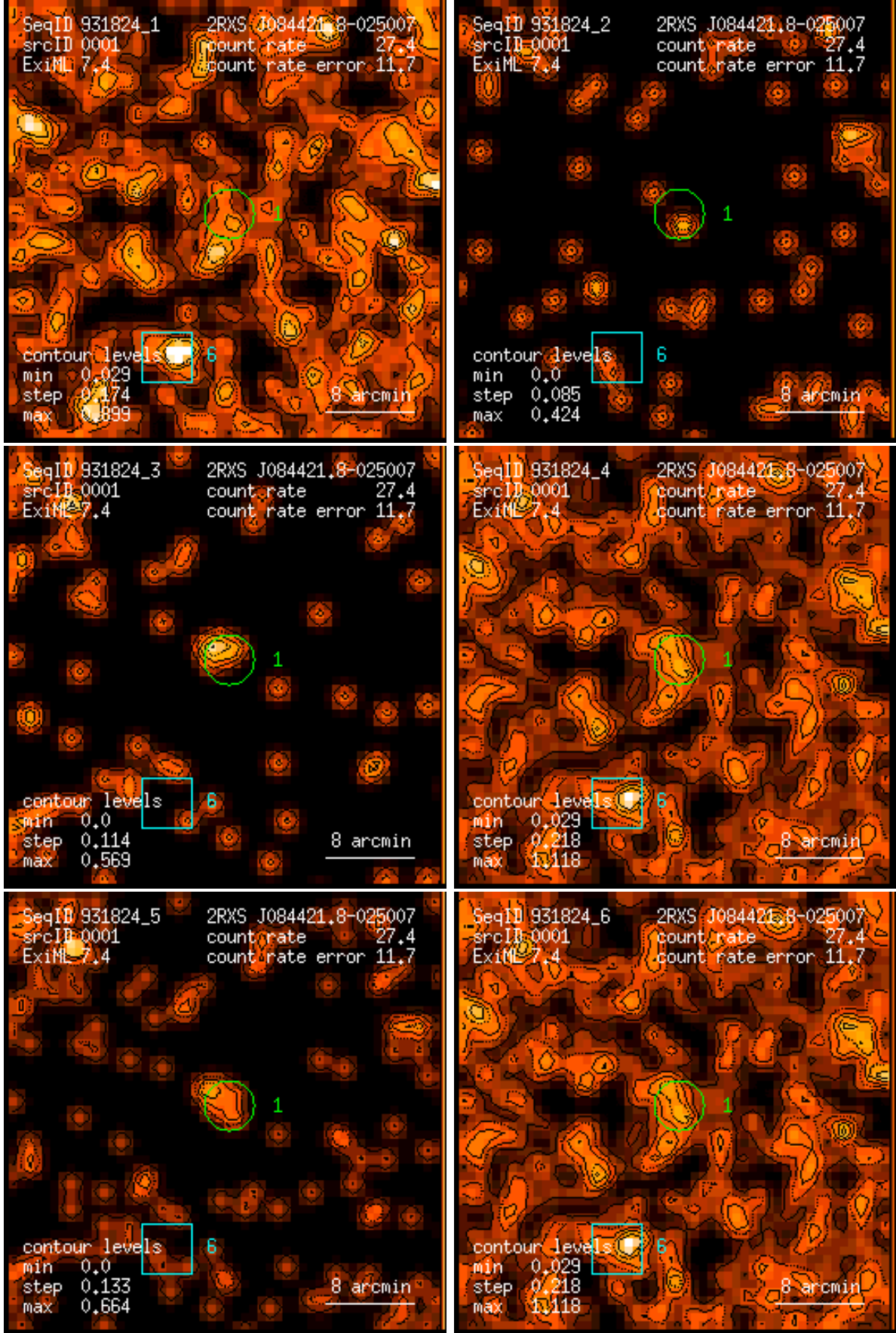
Figure 1: RASS 931824: detection 0001: band rate images, Gaussian filter: (1) PSPC channels 11 – 41, (2) 52 – 90, (3) 91 – 201, (4) 11 – 235, (5) 52 – 201, (6) 11 – 201. Broad band rates in counts/ks. Band rate contour levels in counts/ks/arcmin 2 .
