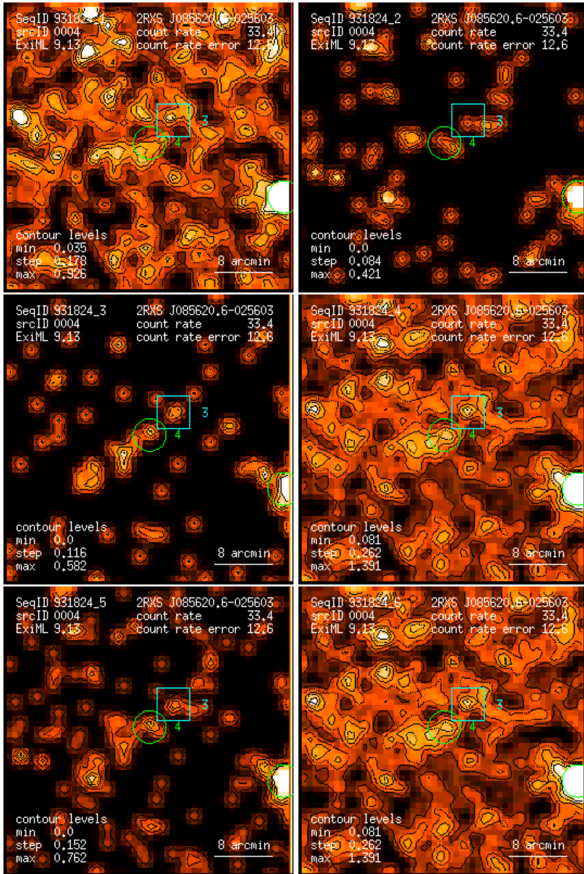
Figure 4: RASS 931824: detection 0004: band rate images, Gaussian filter: (1) PSPC channels 11 – 41, (2) 52 – 90, (3) 91 – 201, (4) 11 – 235, (5) 52 – 201, (6) 11 – 201. Broad band rates in counts/ks. Band rate contour levels in counts/ks/arcmin 2 .
