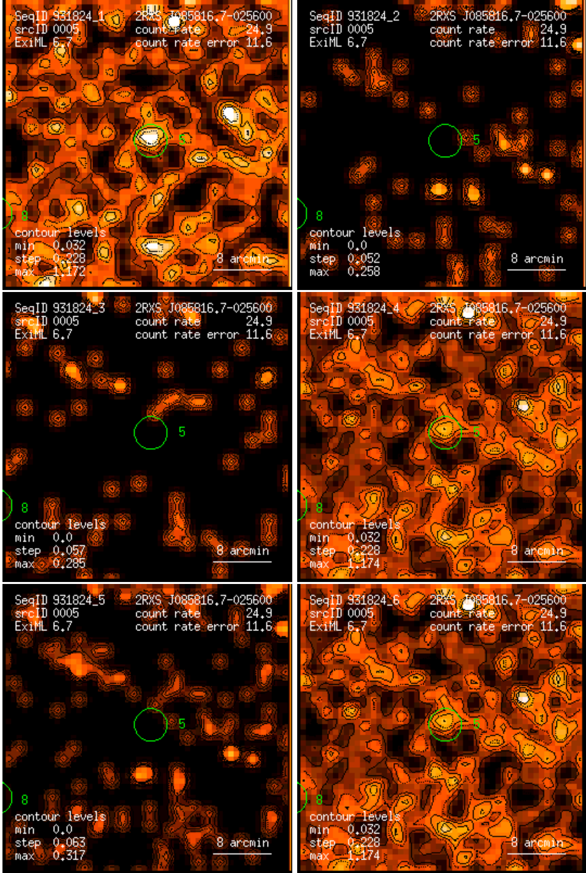
Figure 5: RASS 931824: detection 0005: band rate images, Gaussian filter: (1) PSPC channels 11 – 41, (2) 52 – 90, (3) 91 – 201, (4) 11 – 235, (5) 52 – 201, (6) 11 – 201. Broad band rates in counts/ks. Band rate contour levels in counts/ks/arcmin 2 .
