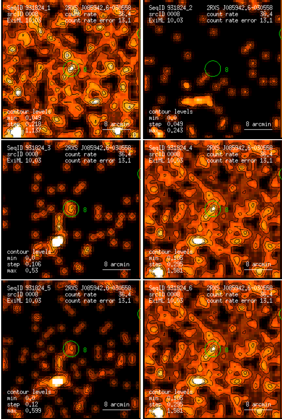
Figure 8: RASS 931824: detection 0008: band rate images, Gaussian filter: (1) PSPC channels 11 – 41, (2) 52 – 90, (3) 91 – 201, (4) 11 – 235, (5) 52 – 201, (6) 11 – 201. Broad band rates in counts/ks. Band rate contour levels in counts/ks/arcmin 2 .
