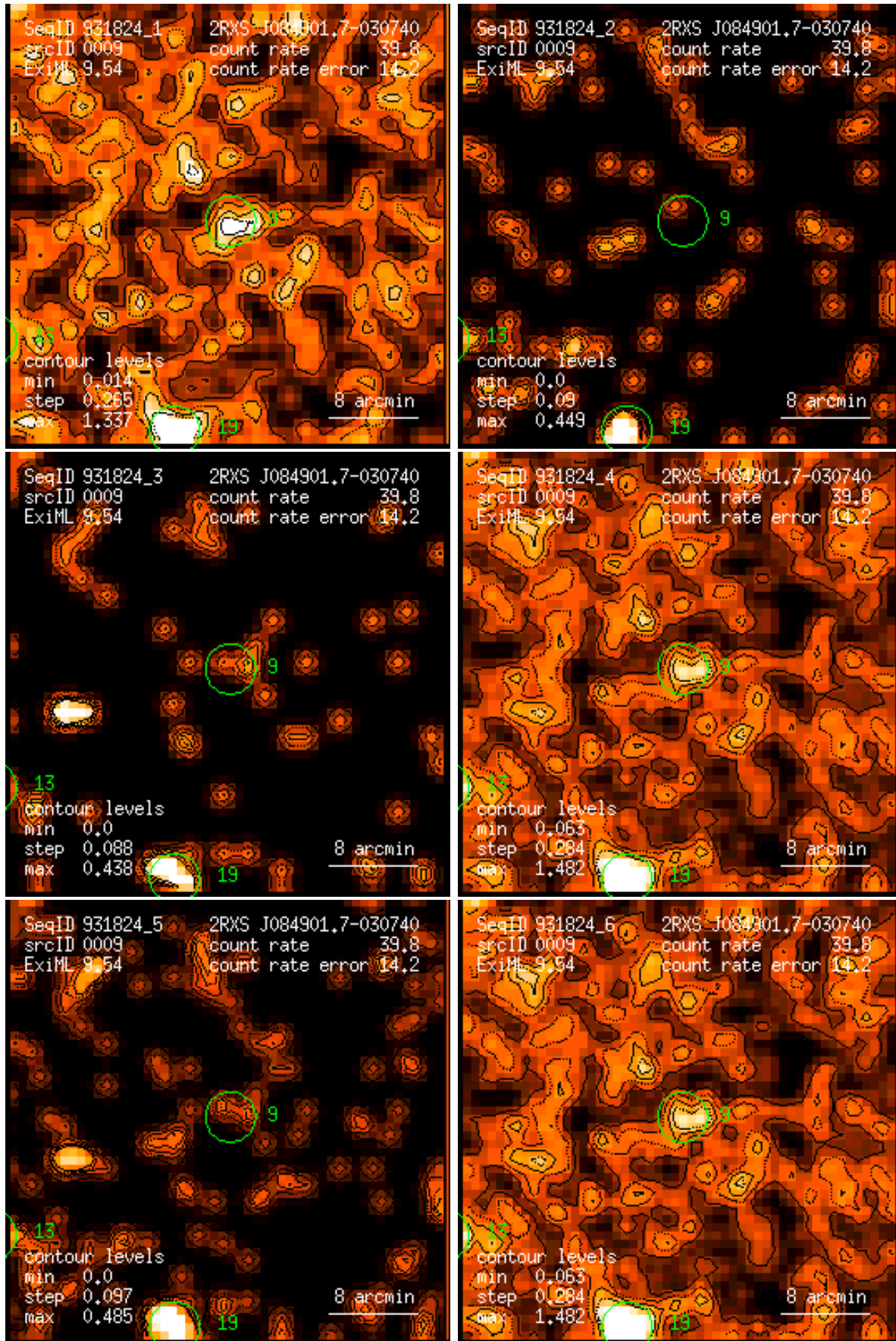
Figure 9: RASS 931824: detection 0009: band rate images, Gaussian filter: (1) PSPC channels 11 – 41, (2) 52 – 90, (3) 91 – 201, (4) 11 – 235, (5) 52 – 201, (6) 11 – 201. Broad band rates in counts/ks. Band rate contour levels in counts/ks/arcmin 2 .
