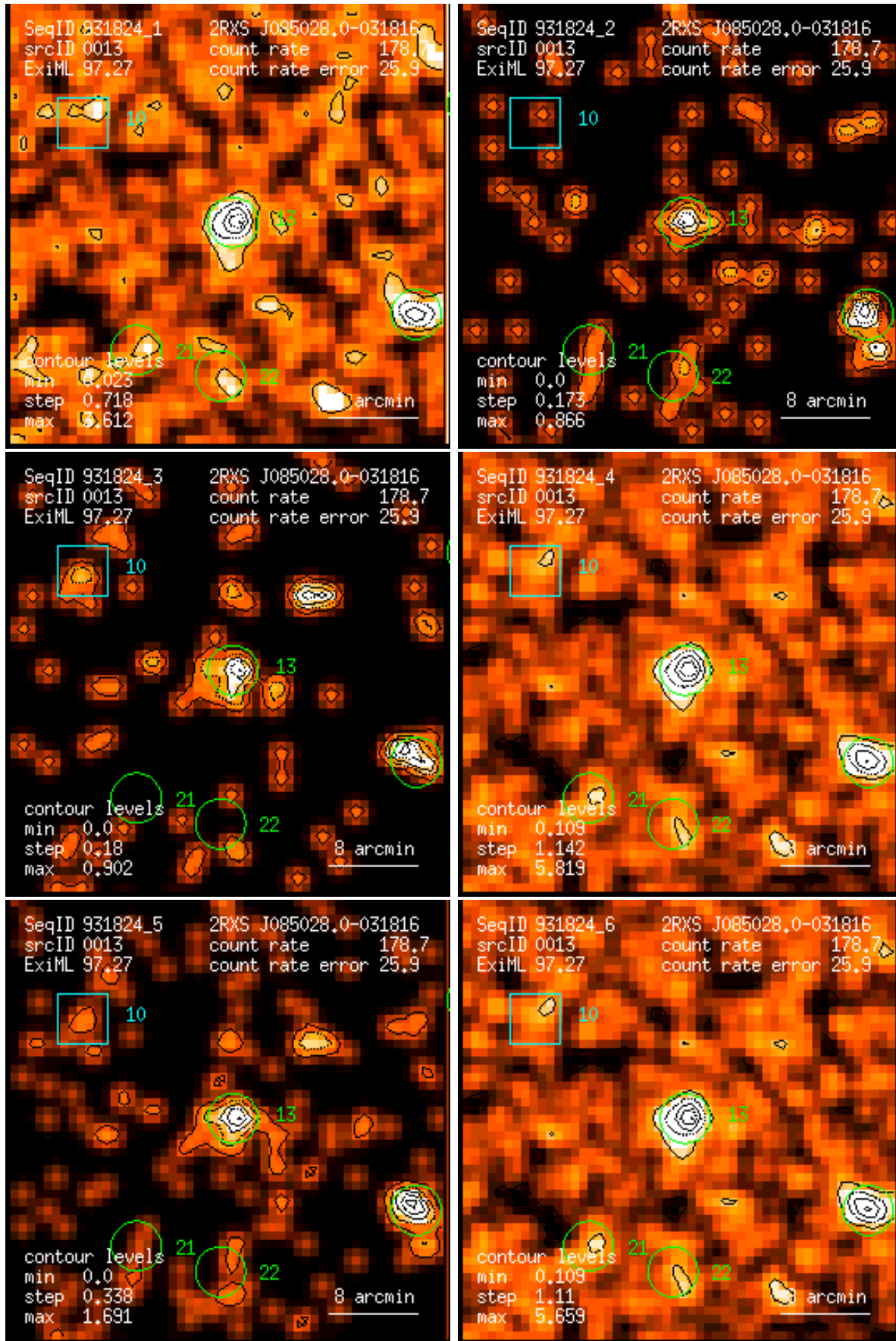
Figure 13: RASS 931824: detection 0013: band rate images, Gaussian filter: (1) PSPC channels 11 – 41, (2) 52 – 90, (3) 91 – 201, (4) 11 – 235, (5) 52 – 201, (6) 11 – 201. Broad band rates in counts/ks. Band rate contour levels in counts/ks/arcmin 2 .
