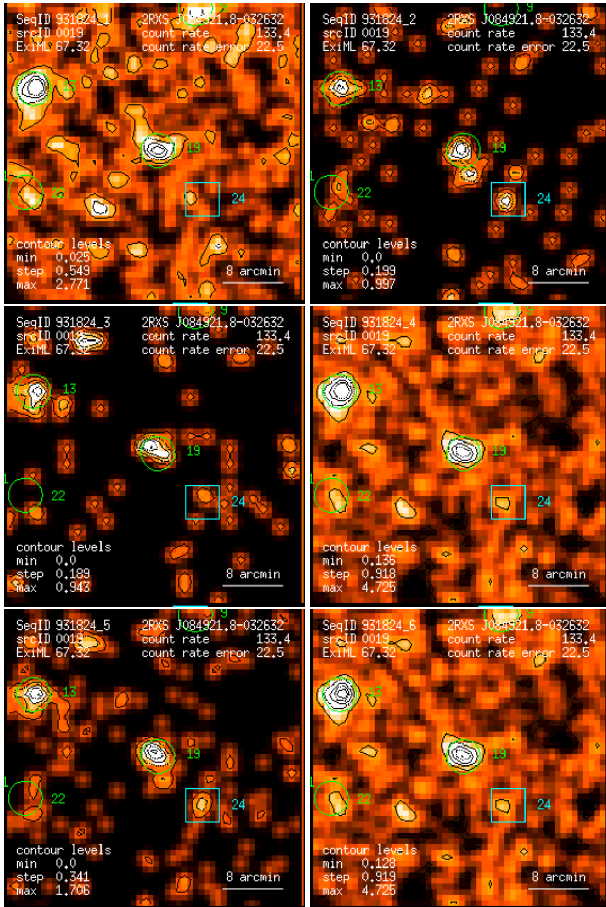
Figure 19: RASS 931824: detection 0019: band rate images, Gaussian filter: (1) PSPC channels 11 – 41, (2) 52 – 90, (3) 91 – 201, (4) 11 – 235, (5) 52 – 201, (6) 11 – 201. Broad band rates in counts/ks. Band rate contour levels in counts/ks/arcmin 2 .
