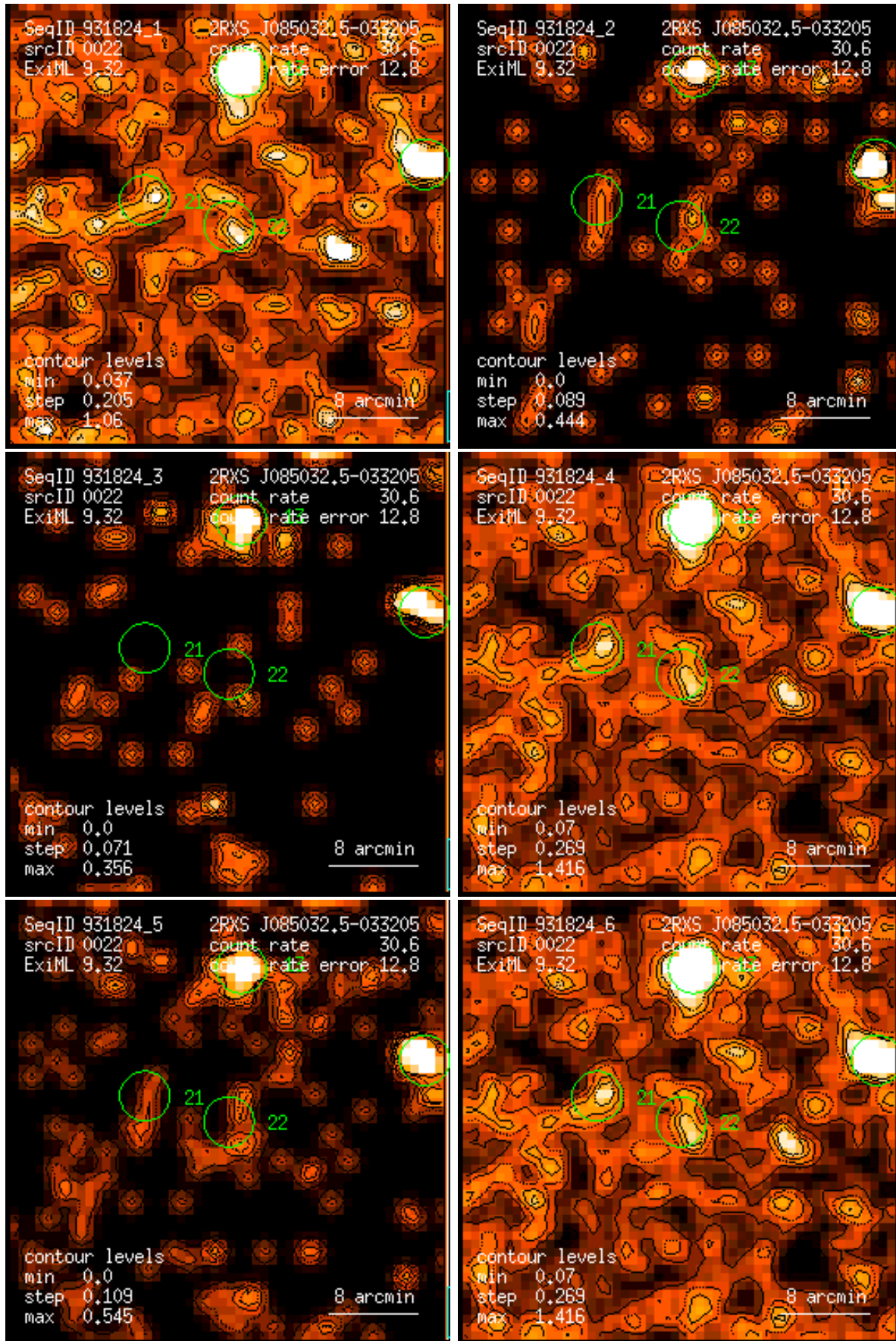
Figure 22: RASS 931824: detection 0022: band rate images, Gaussian filter: (1) PSPC channels 11 – 41, (2) 52 – 90, (3) 91 – 201, (4) 11 – 235, (5) 52 – 201, (6) 11 – 201. Broad band rates in counts/ks. Band rate contour levels in counts/ks/arcmin 2 .
