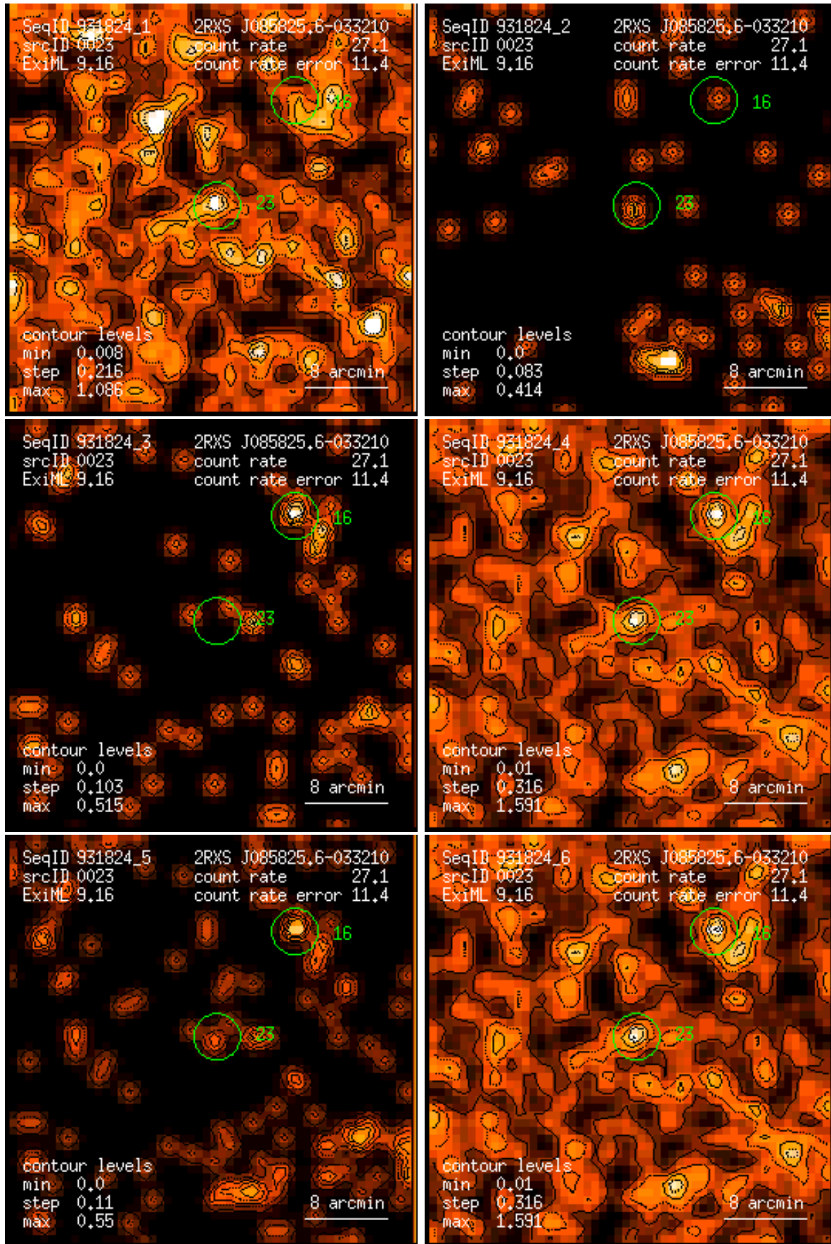
Figure 23: RASS 931824: detection 0023: band rate images, Gaussian filter: (1) PSPC channels 11 – 41, (2) 52 – 90, (3) 91 – 201, (4) 11 – 235, (5) 52 – 201, (6) 11 – 201. Broad band rates in counts/ks. Band rate contour levels in counts/ks/arcmin 2 .
