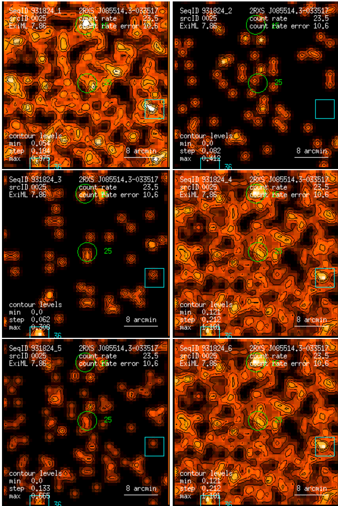
Figure 25: RASS 931824: detection 0025: band rate images, Gaussian filter: (1) PSPC channels 11 – 41, (2) 52 – 90, (3) 91 – 201, (4) 11 – 235, (5) 52 – 201, (6) 11 – 201. Broad band rates in counts/ks. Band rate contour levels in counts/ks/arcmin 2 .
