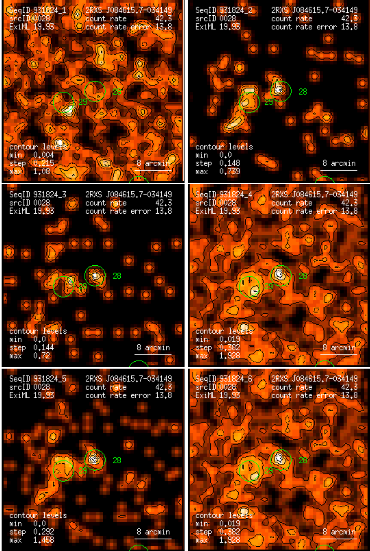
Figure 28: RASS 931824: detection 0028: band rate images, Gaussian filter: (1) PSPC channels 11 – 41, (2) 52 – 90, (3) 91 – 201, (4) 11 – 235, (5) 52 – 201, (6) 11 – 201. Broad band rates in counts/ks. Band rate contour levels in counts/ks/arcmin 2 .
