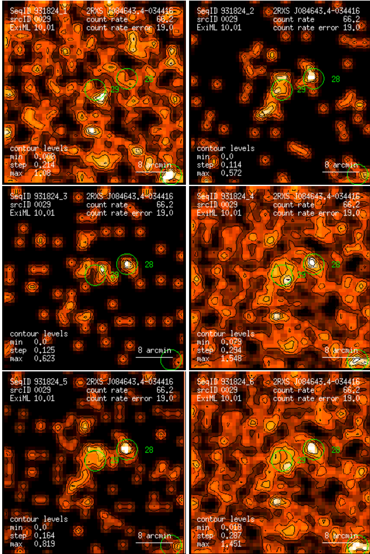
Figure 29: RASS 931824: detection 0029: band rate images, Gaussian filter: (1) PSPC channels 11 – 41, (2) 52 – 90, (3) 91 – 201, (4) 11 – 235, (5) 52 – 201, (6) 11 – 201. Broad band rates in counts/ks. Band rate contour levels in counts/ks/arcmin 2 .
