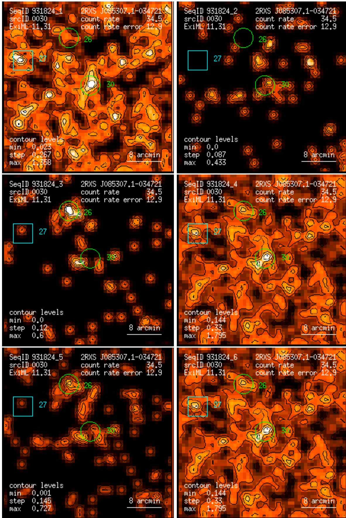
Figure 30: RASS 931824: detection 0030: band rate images, Gaussian filter: (1) PSPC channels 11 – 41, (2) 52 – 90, (3) 91 – 201, (4) 11 – 235, (5) 52 – 201, (6) 11 – 201. Broad band rates in counts/ks. Band rate contour levels in counts/ks/arcmin 2 .
