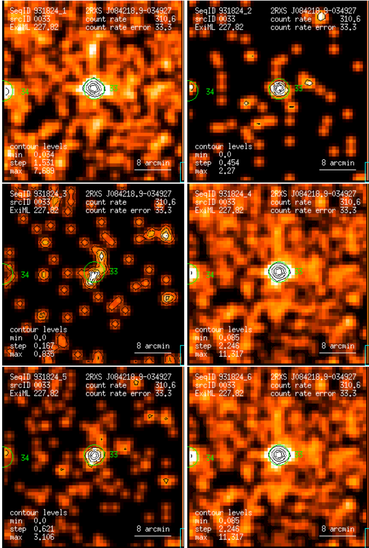
Figure 33: RASS 931824: detection 0033: band rate images, Gaussian filter: (1) PSPC channels 11 – 41, (2) 52 – 90, (3) 91 – 201, (4) 11 – 235, (5) 52 – 201, (6) 11 – 201. Broad band rates in counts/ks. Band rate contour levels in counts/ks/arcmin 2 .
