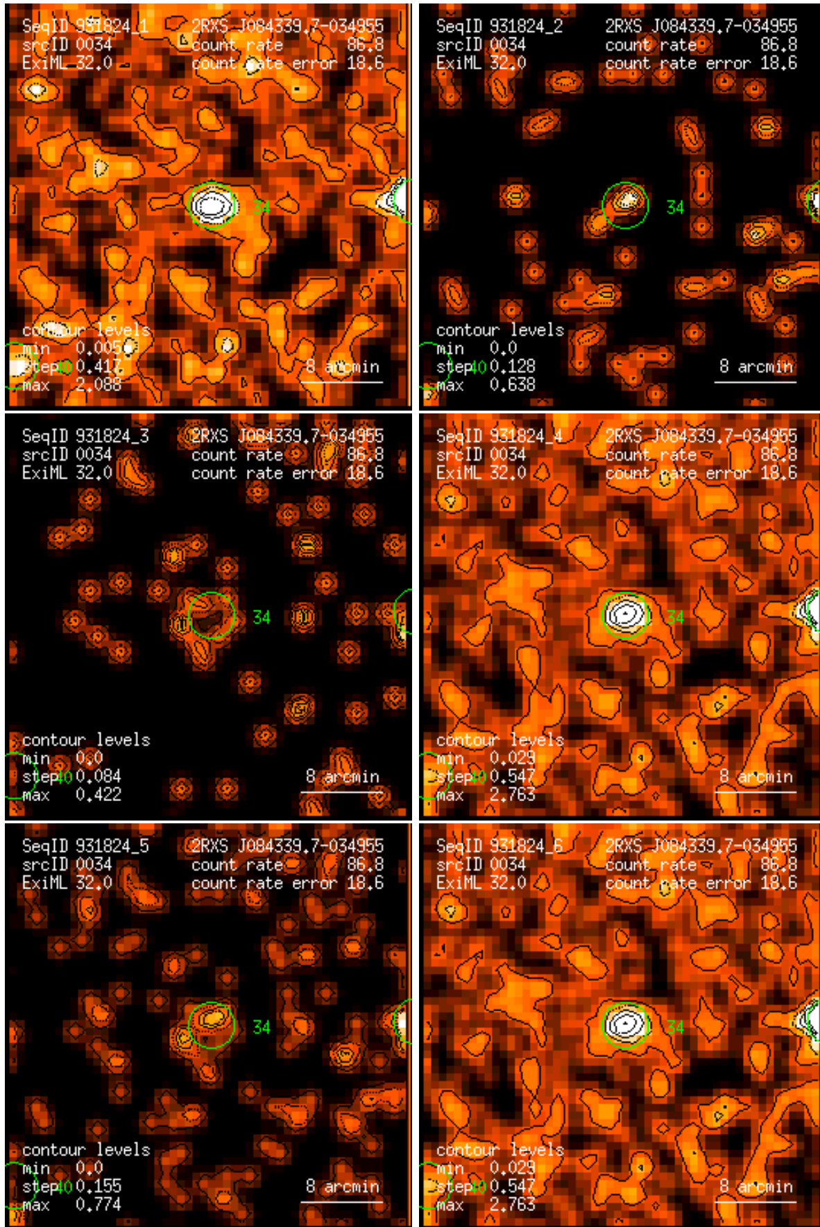
Figure 34: RASS 931824: detection 0034: band rate images, Gaussian filter: (1) PSPC channels 11 – 41, (2) 52 – 90, (3) 91 – 201, (4) 11 – 235, (5) 52 – 201, (6) 11 – 201. Broad band rates in counts/ks. Band rate contour levels in counts/ks/arcmin 2 .
