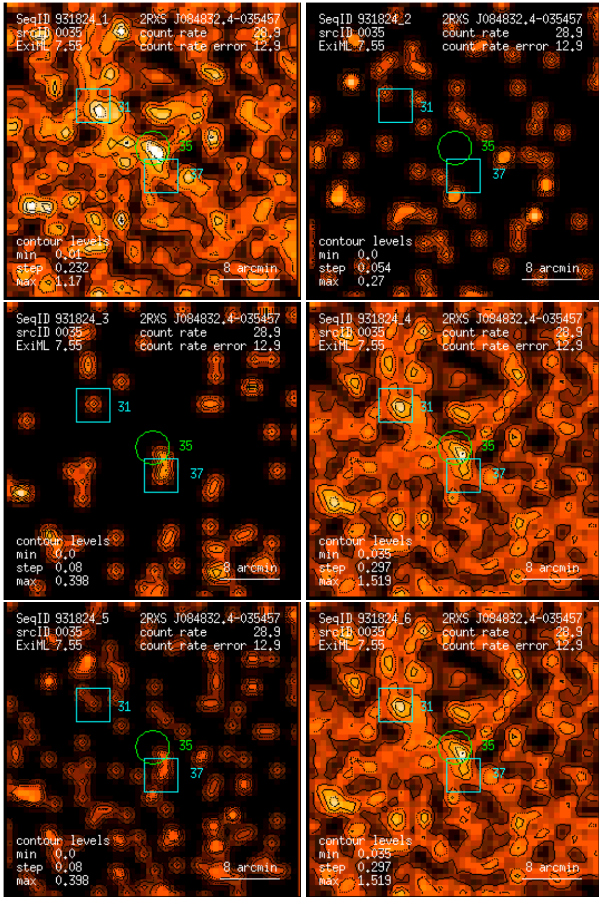
Figure 35: RASS 931824: detection 0035: band rate images, Gaussian filter: (1) PSPC channels 11 – 41, (2) 52 – 90, (3) 91 – 201, (4) 11 – 235, (5) 52 – 201, (6) 11 – 201. Broad band rates in counts/ks. Band rate contour levels in counts/ks/arcmin 2 .
