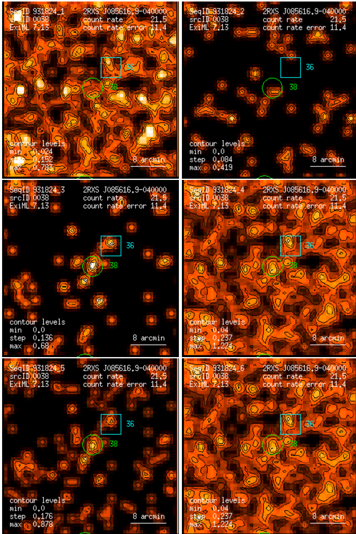
Figure 38: RASS 931824: detection 0038: band rate images, Gaussian filter: (1) PSPC channels 11 – 41, (2) 52 – 90, (3) 91 – 201, (4) 11 – 235, (5) 52 – 201, (6) 11 – 201. Broad band rates in counts/ks. Band rate contour levels in counts/ks/arcmin 2 .
