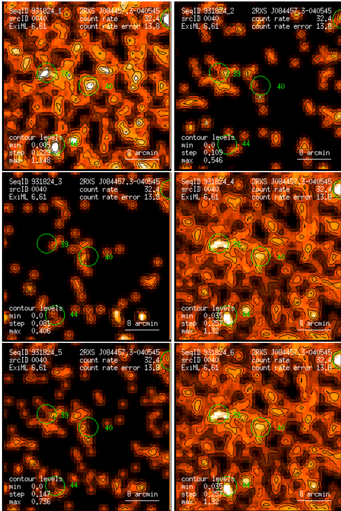
Figure 40: RASS 931824: detection 0040: band rate images, Gaussian filter: (1) PSPC channels 11 – 41, (2) 52 – 90, (3) 91 – 201, (4) 11 – 235, (5) 52 – 201, (6) 11 – 201. Broad band rates in counts/ks. Band rate contour levels in counts/ks/arcmin 2 .
