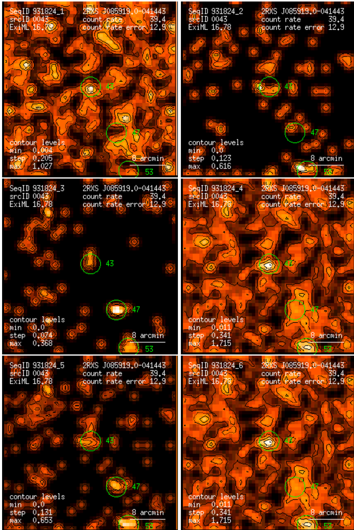
Figure 43: RASS 931824: detection 0043: band rate images, Gaussian filter: (1) PSPC channels 11 – 41, (2) 52 – 90, (3) 91 – 201, (4) 11 – 235, (5) 52 – 201, (6) 11 – 201. Broad band rates in counts/ks. Band rate contour levels in counts/ks/arcmin 2 .
