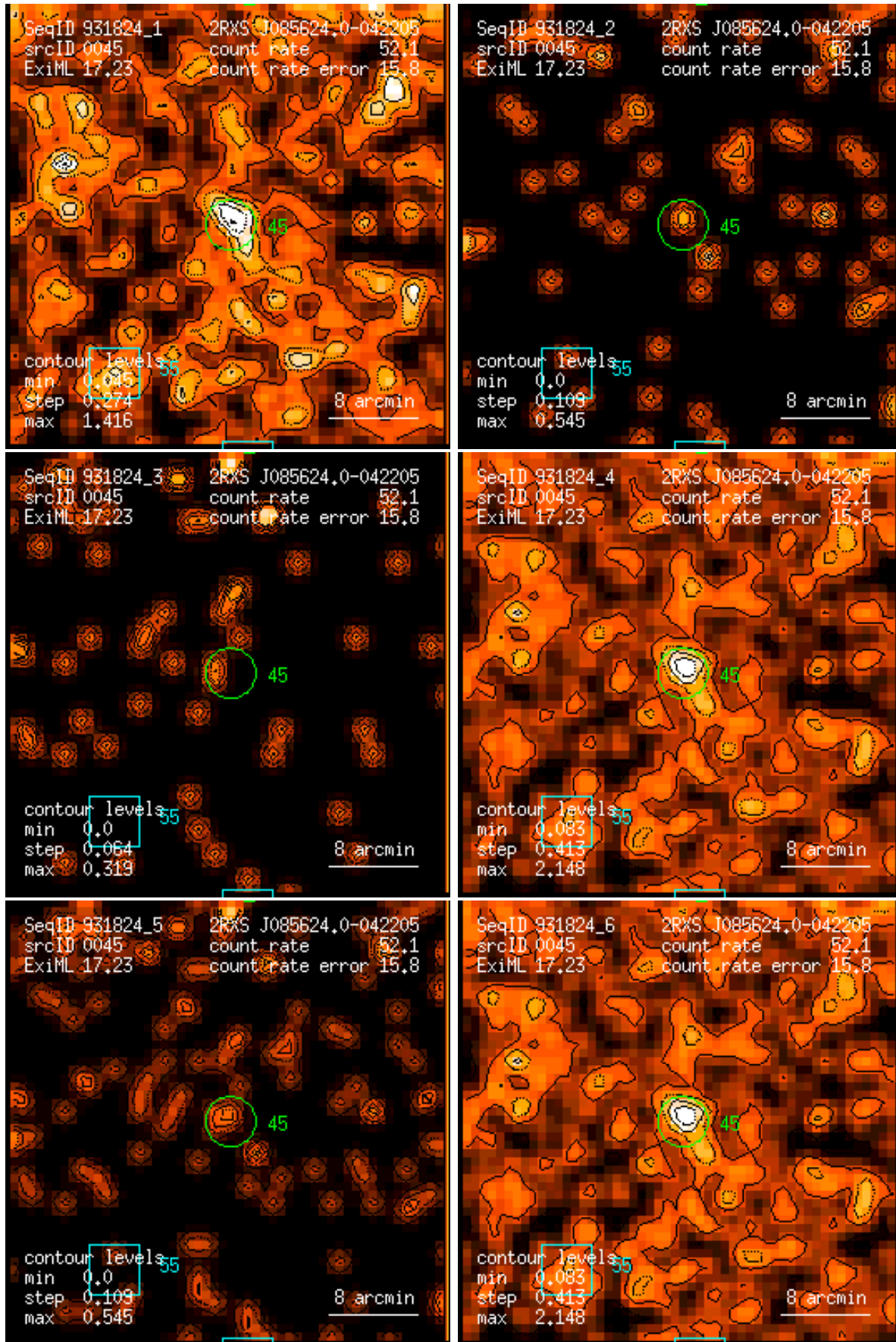
Figure 45: RASS 931824: detection 0045: band rate images, Gaussian filter: (1) PSPC channels 11 – 41, (2) 52 – 90, (3) 91 – 201, (4) 11 – 235, (5) 52 – 201, (6) 11 – 201. Broad band rates in counts/ks. Band rate contour levels in counts/ks/arcmin 2 .
