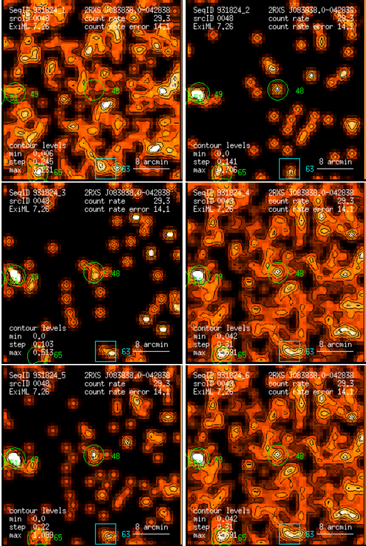
Figure 48: RASS 931824: detection 0048: band rate images, Gaussian filter: (1) PSPC channels 11 – 41, (2) 52 – 90, (3) 91 – 201, (4) 11 – 235, (5) 52 – 201, (6) 11 – 201. Broad band rates in counts/ks. Band rate contour levels in counts/ks/arcmin 2 .
