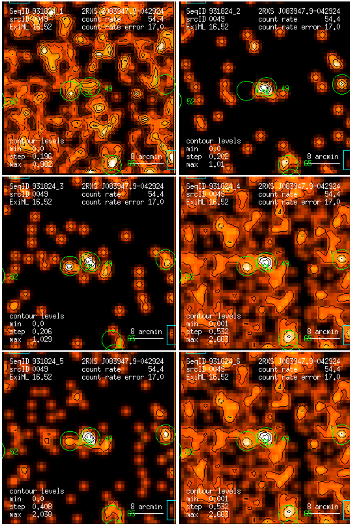
Figure 49: RASS 931824: detection 0049: band rate images, Gaussian filter: (1) PSPC channels 11 – 41, (2) 52 – 90, (3) 91 – 201, (4) 11 – 235, (5) 52 – 201, (6) 11 – 201. Broad band rates in counts/ks. Band rate contour levels in counts/ks/arcmin 2 .
