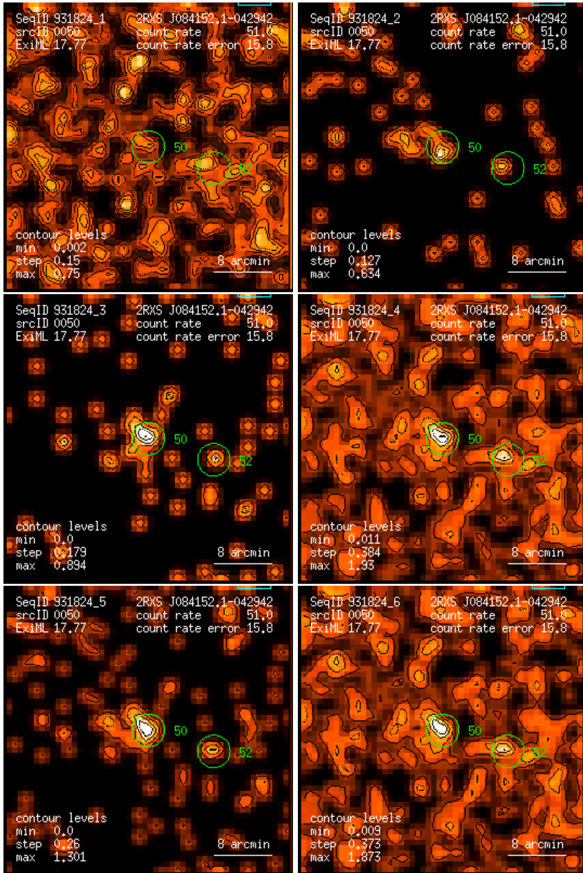
Figure 50: RASS 931824: detection 0050: band rate images, Gaussian filter: (1) PSPC channels 11 – 41, (2) 52 – 90, (3) 91 – 201, (4) 11 – 235, (5) 52 – 201, (6) 11 – 201. Broad band rates in counts/ks. Band rate contour levels in counts/ks/arcmin 2 .
