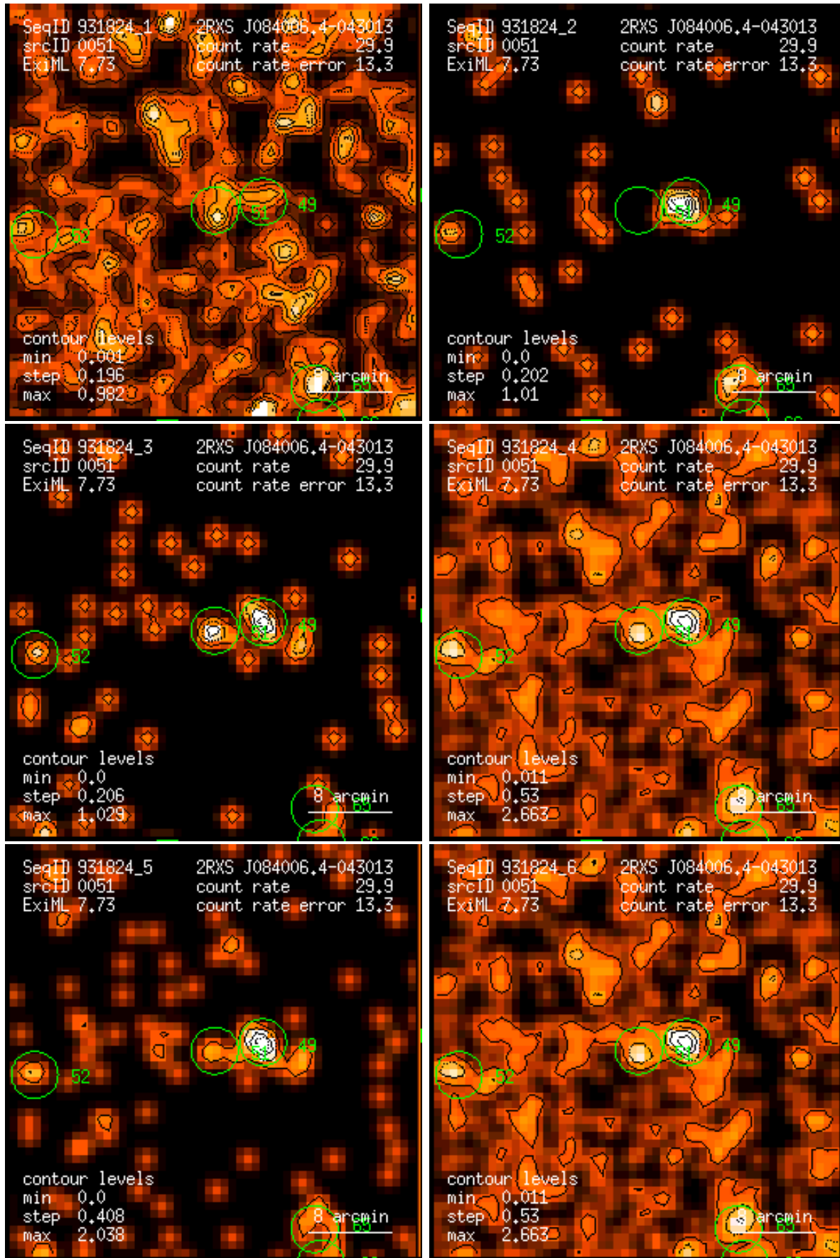
Figure 51: RASS 931824: detection 0051: band rate images, Gaussian filter: (1) PSPC channels 11 – 41, (2) 52 – 90, (3) 91 – 201, (4) 11 – 235, (5) 52 – 201, (6) 11 – 201. Broad band rates in counts/ks. Band rate contour levels in counts/ks/arcmin 2 .
