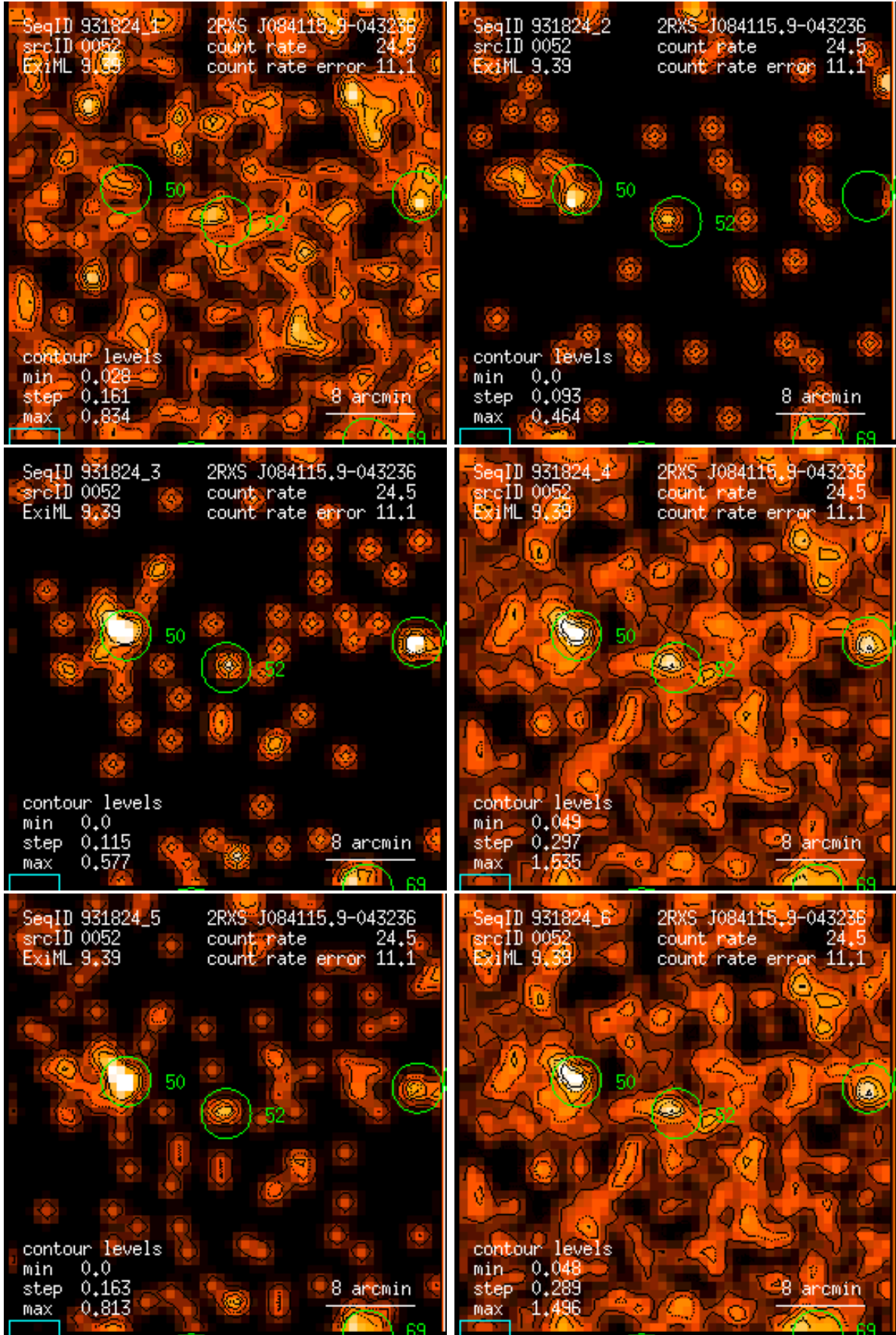
Figure 52: RASS 931824: detection 0052: band rate images, Gaussian filter: (1) PSPC channels 11 – 41, (2) 52 – 90, (3) 91 – 201, (4) 11 – 235, (5) 52 – 201, (6) 11 – 201. Broad band rates in counts/ks. Band rate contour levels in counts/ks/arcmin 2 .
