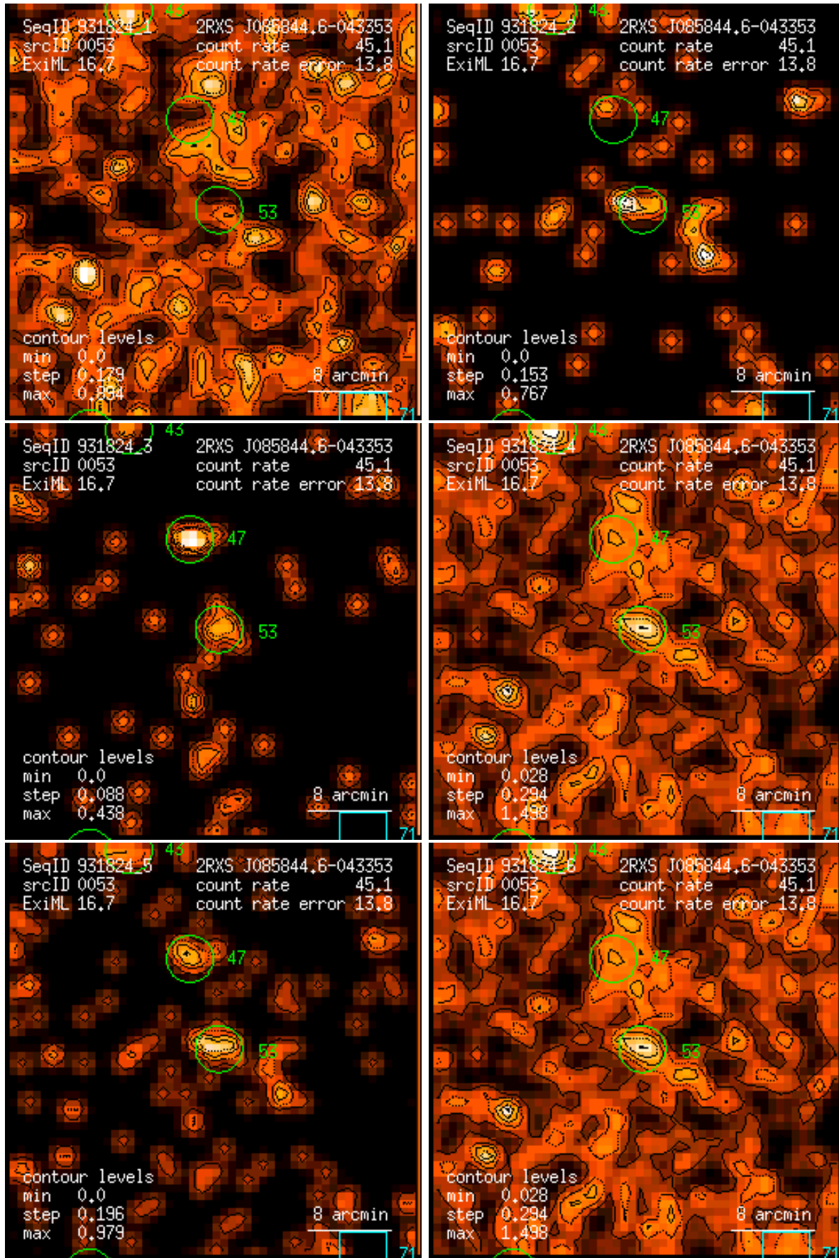
Figure 53: RASS 931824: detection 0053: band rate images, Gaussian filter: (1) PSPC channels 11 – 41, (2) 52 – 90, (3) 91 – 201, (4) 11 – 235, (5) 52 – 201, (6) 11 – 201. Broad band rates in counts/ks. Band rate contour levels in counts/ks/arcmin 2 .
