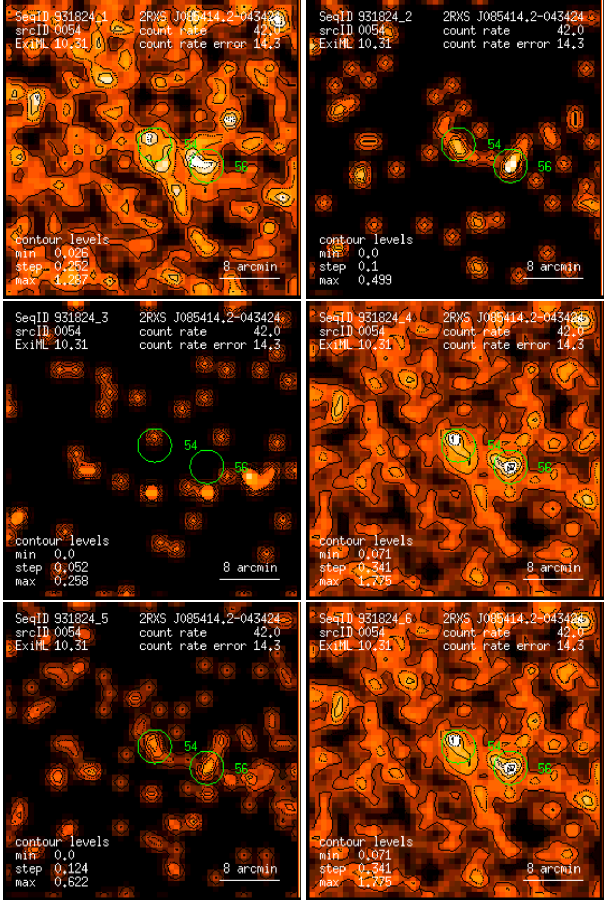
Figure 54: RASS 931824: detection 0054: band rate images, Gaussian filter: (1) PSPC channels 11 – 41, (2) 52 – 90, (3) 91 – 201, (4) 11 – 235, (5) 52 – 201, (6) 11 – 201. Broad band rates in counts/ks. Band rate contour levels in counts/ks/arcmin 2 .
