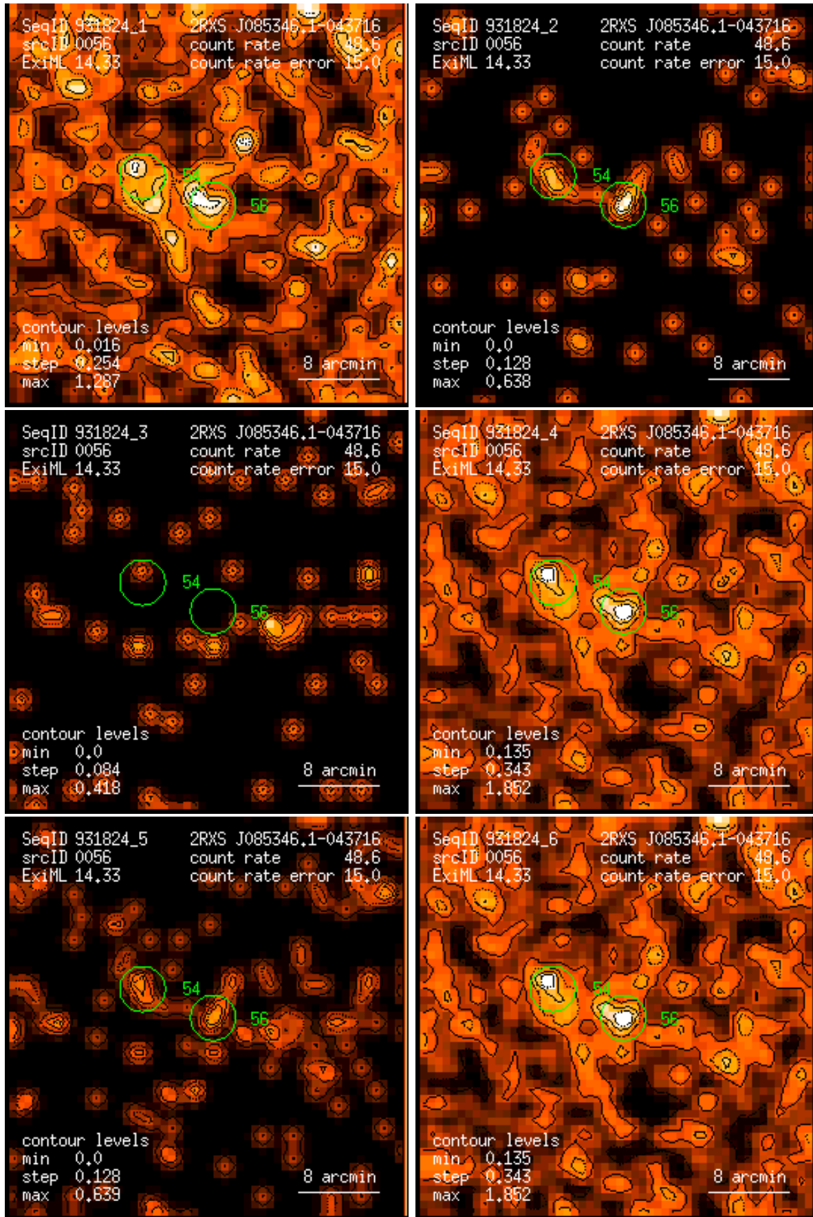
Figure 56: RASS 931824: detection 0056: band rate images, Gaussian filter: (1) PSPC channels 11 – 41, (2) 52 – 90, (3) 91 – 201, (4) 11 – 235, (5) 52 – 201, (6) 11 – 201. Broad band rates in counts/ks. Band rate contour levels in counts/ks/arcmin 2 .
